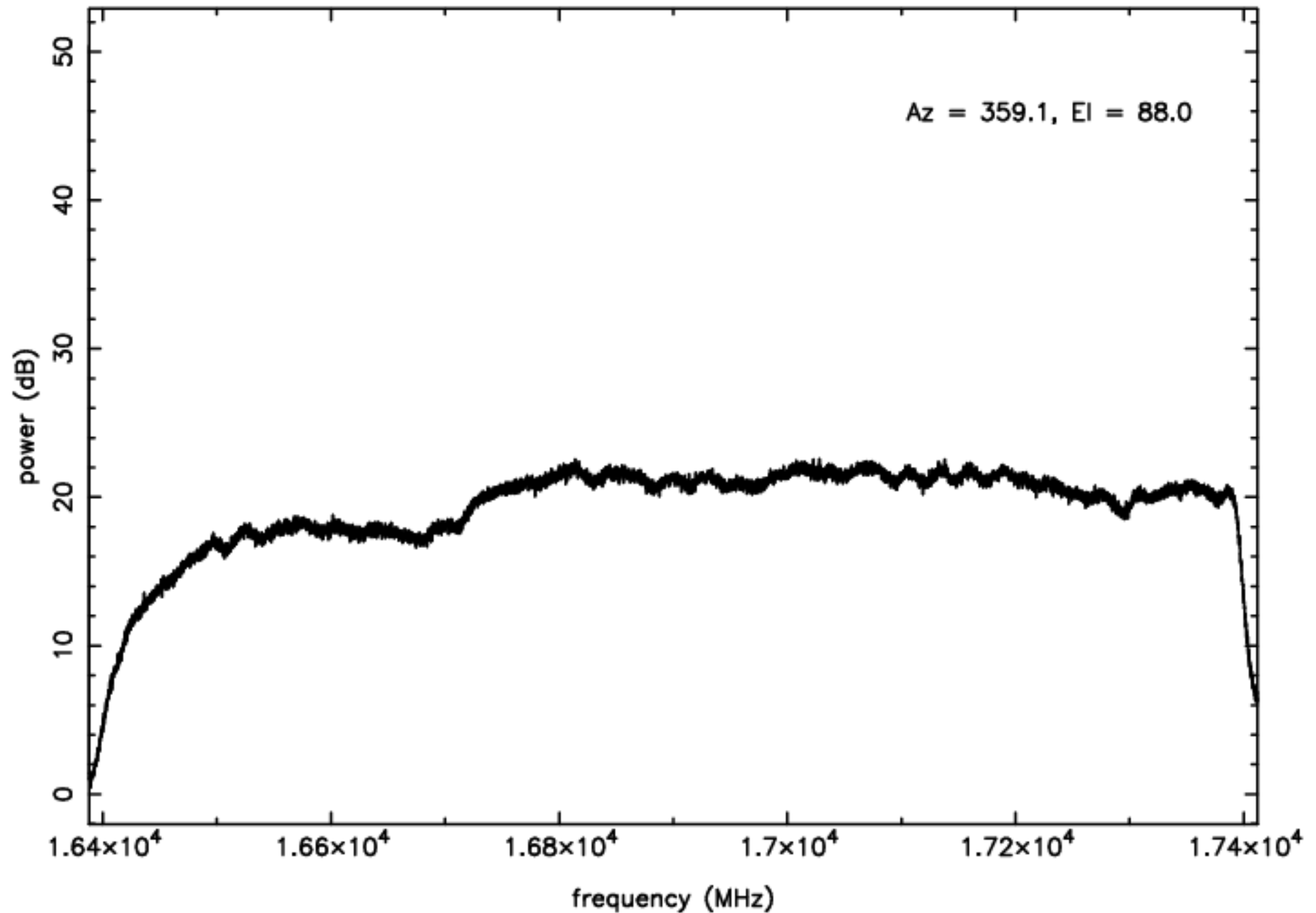
Ku-band RFI plot (mean power) – IF B – ea22
