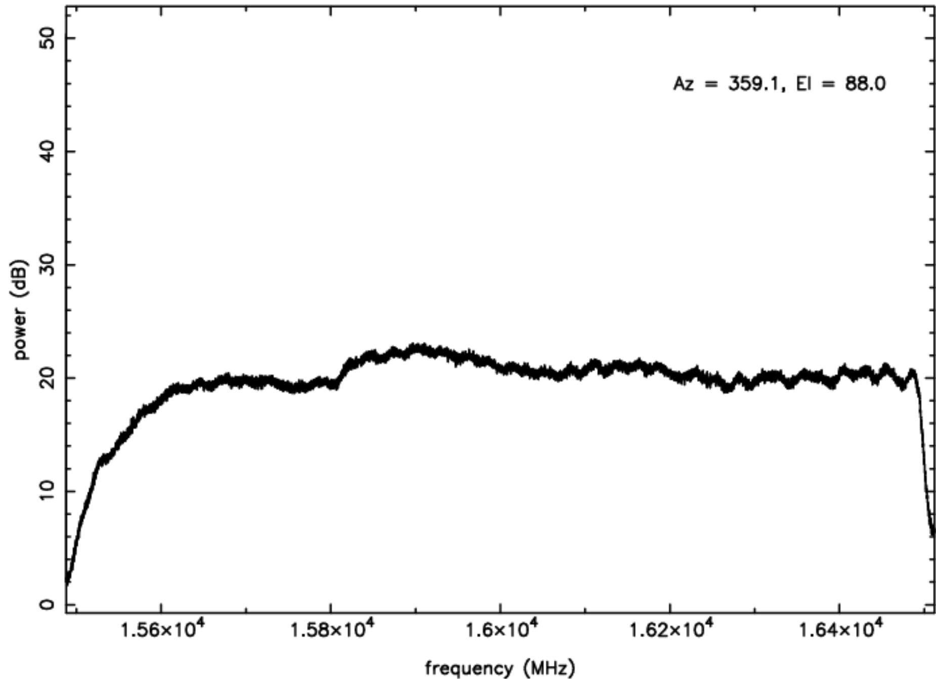
Ku-band RFI plot (mean power) – IF B – ea22
