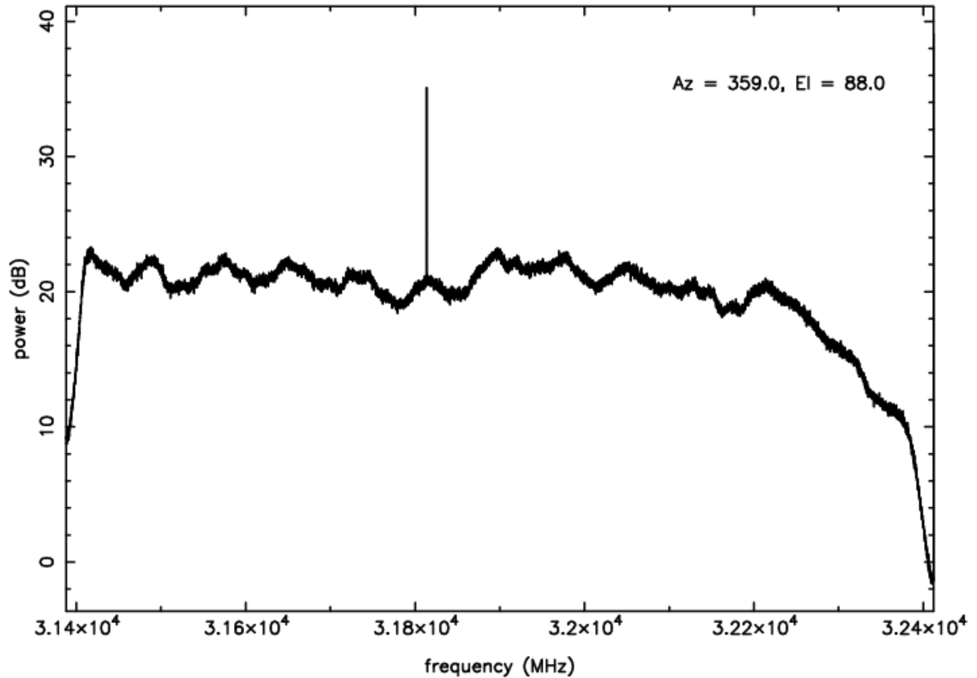
Ka-band RFI plot (mean power) - IF D - ea22
