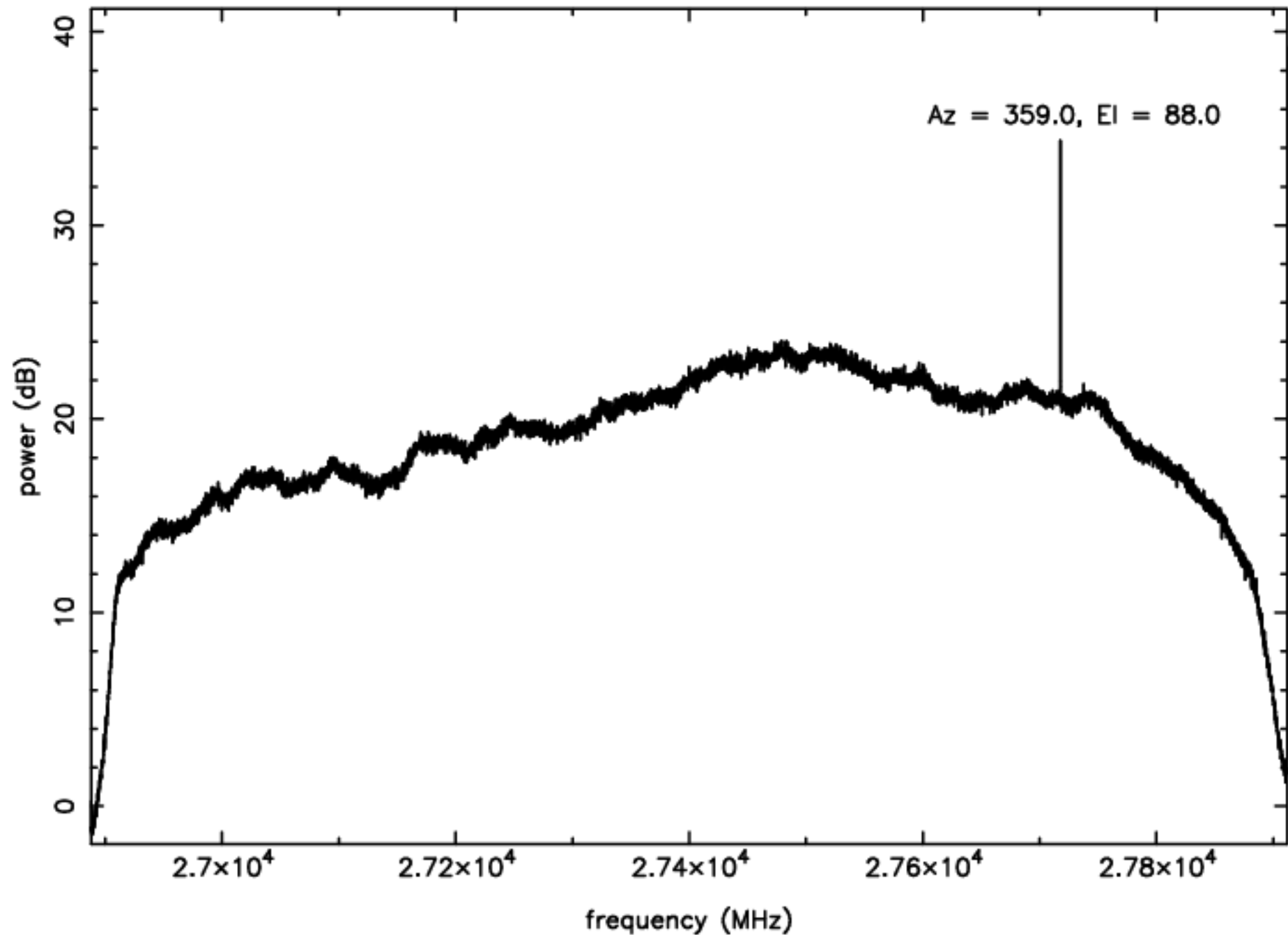
Ka-band RFI plot (mean power) – IF D – ea22
