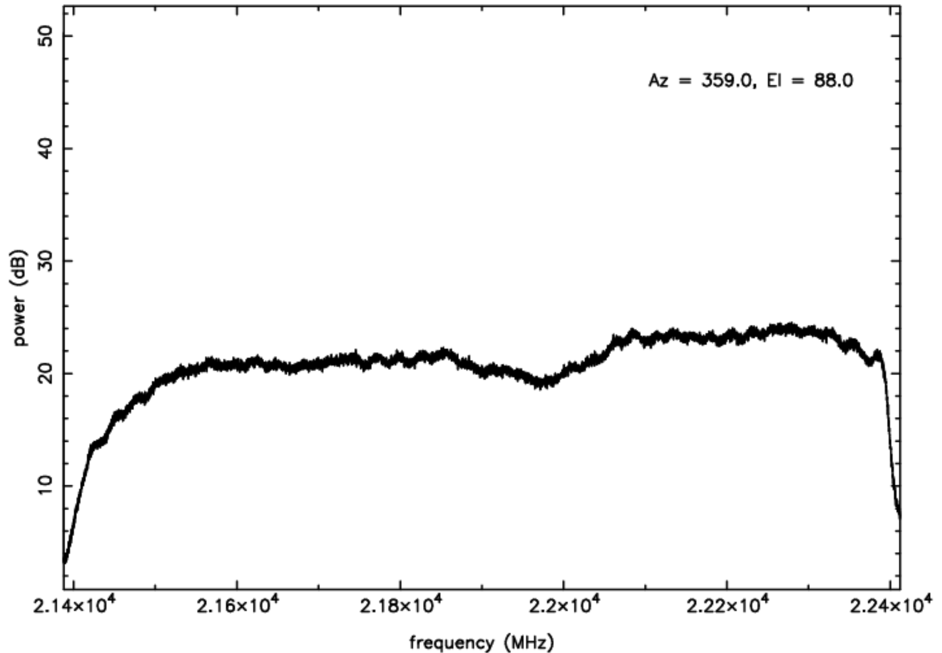
K-band RFI plot (mean power) – IF B – ea22
