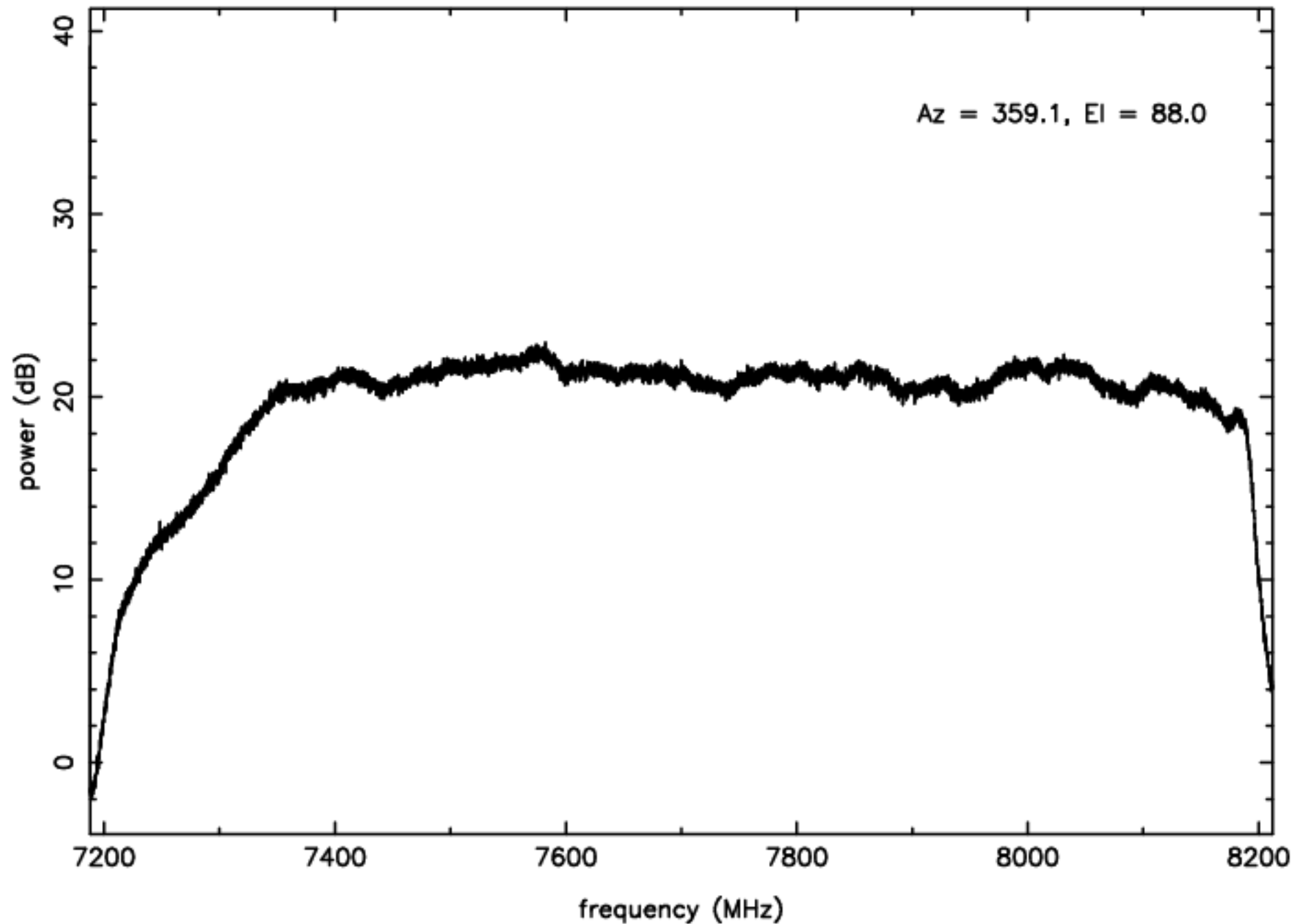
C-band RFI plot (mean power) – IF D – ea22
