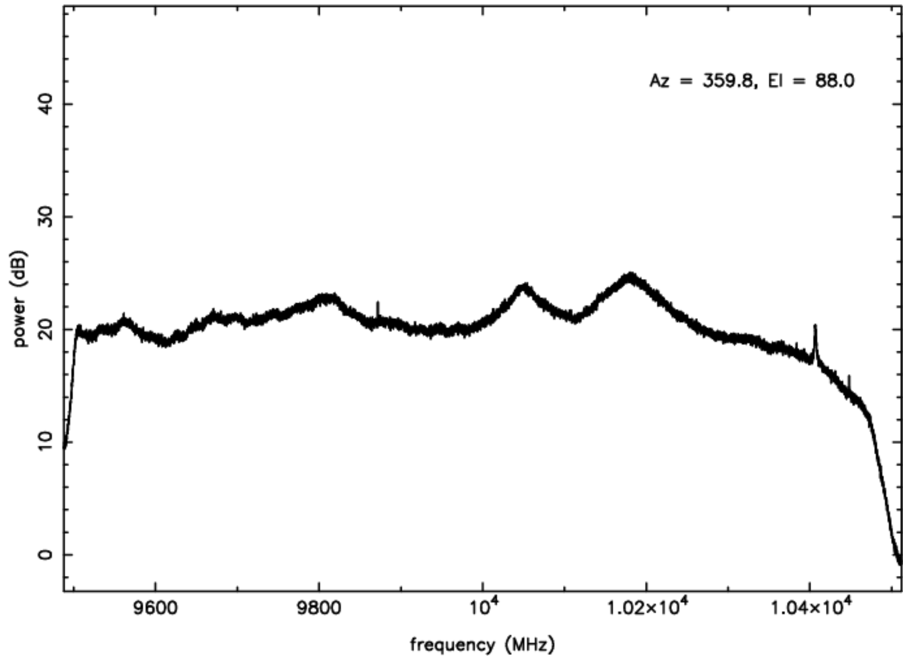
X-band RFI plot (mean power) – IF B – ea10
