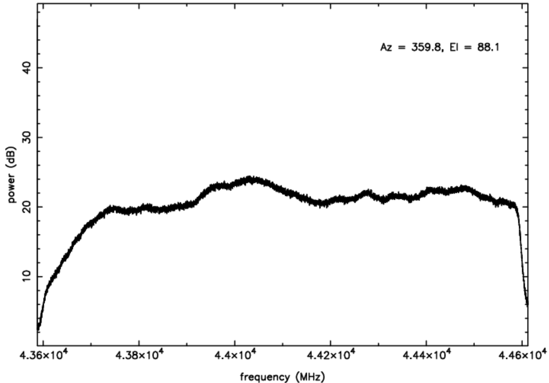
Q-band RFI plot (mean power) – IF D – ea10
