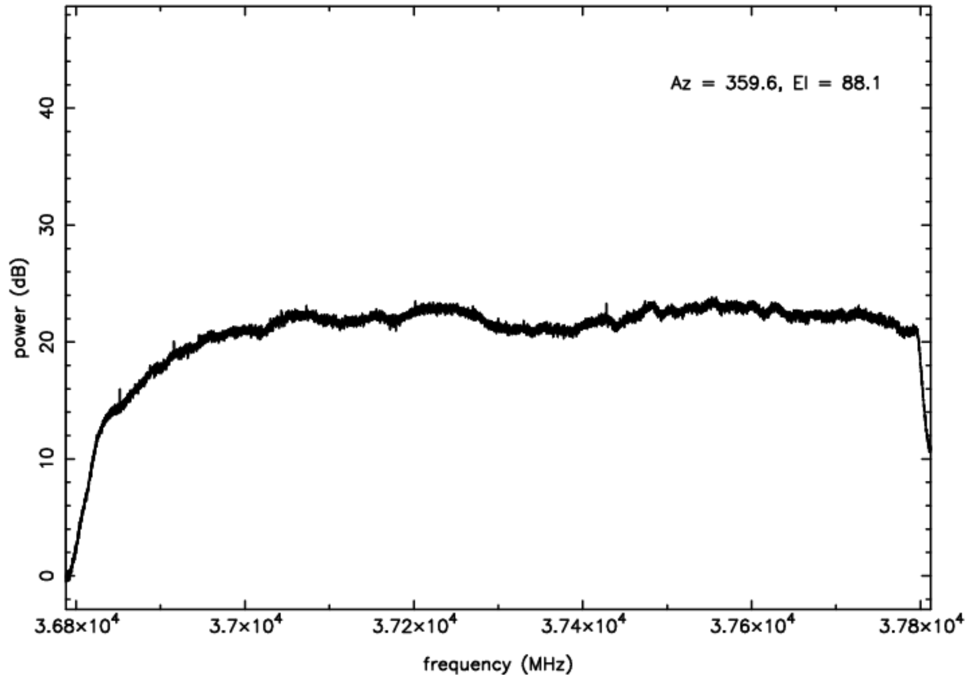
Ka-band RFI plot (mean power) – IF B – ea10
