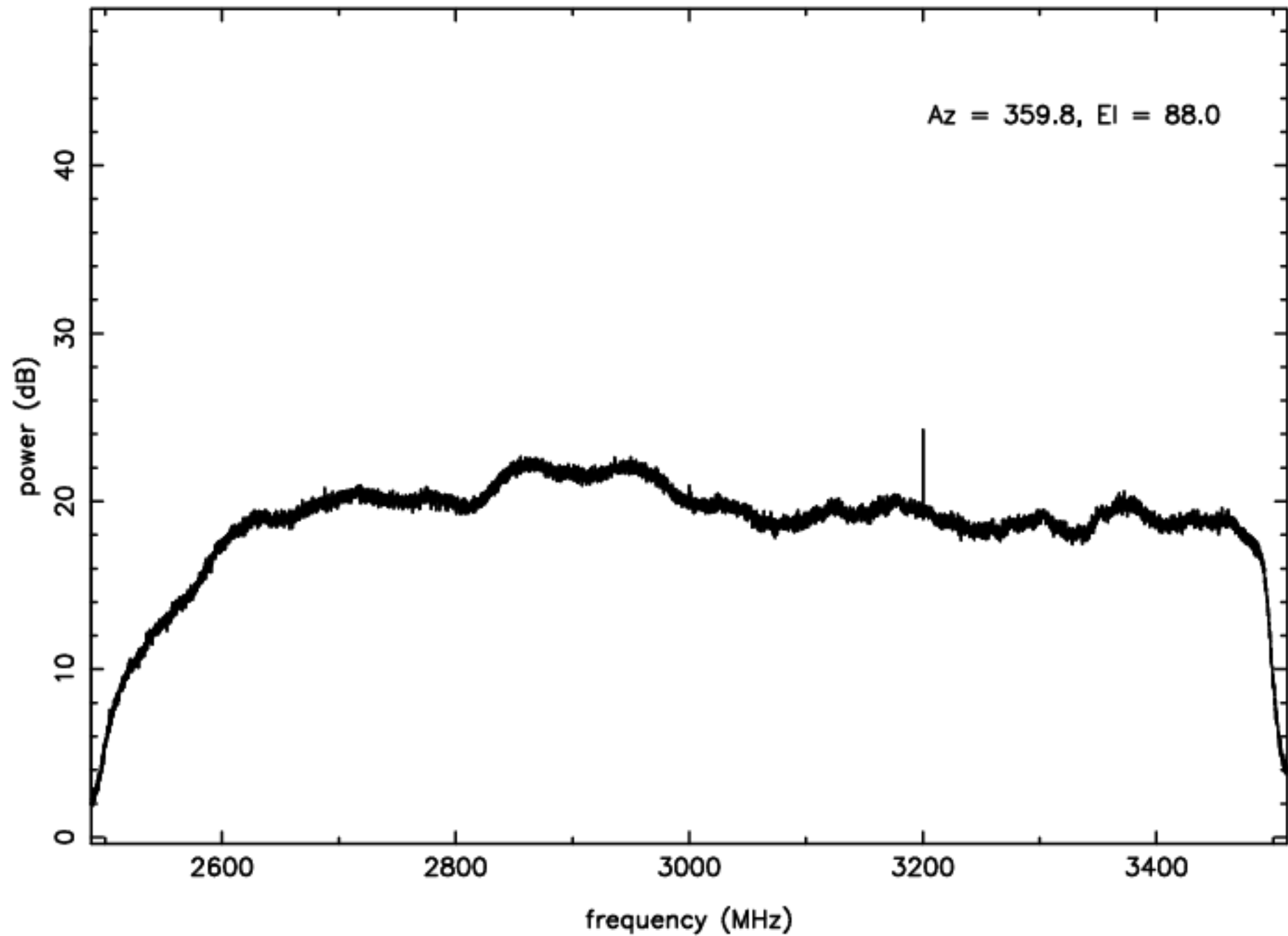
S-band RFI plot (mean power) – IF D – ea10
