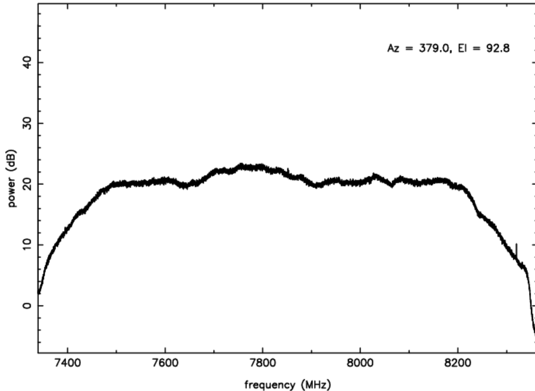
C-band RFI plot (mean power) – IF D – ea10
