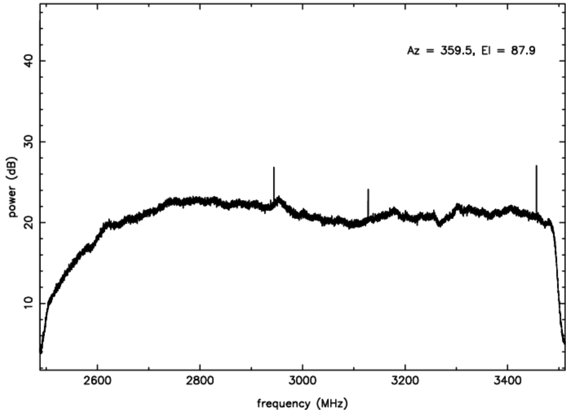
S-band RFI plot (mean power) – IF D – ea07
