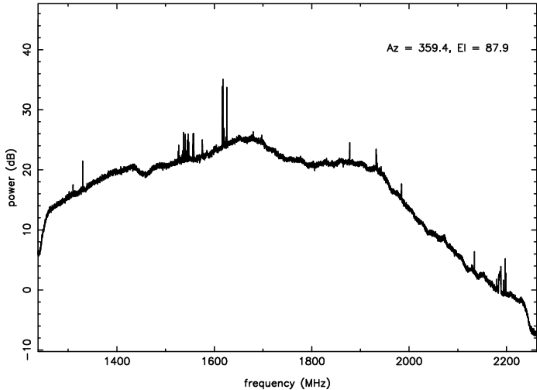
L-band RFI plot (mean power) – IF D – ea07
