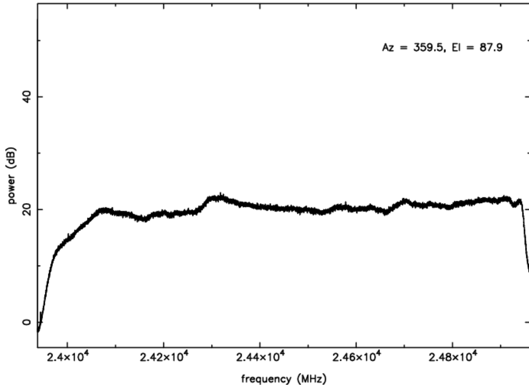
K-band RFI plot (mean power) – IF B – ea07
