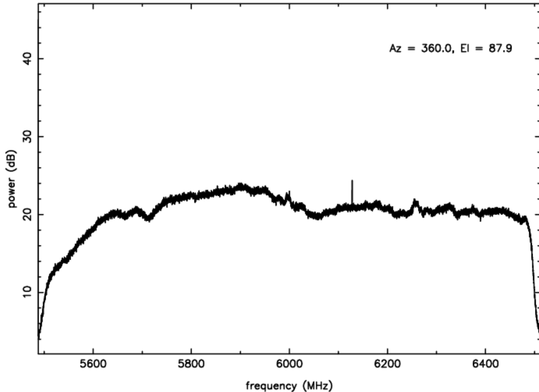
C-band RFI plot (mean power) – IF D – ea07
