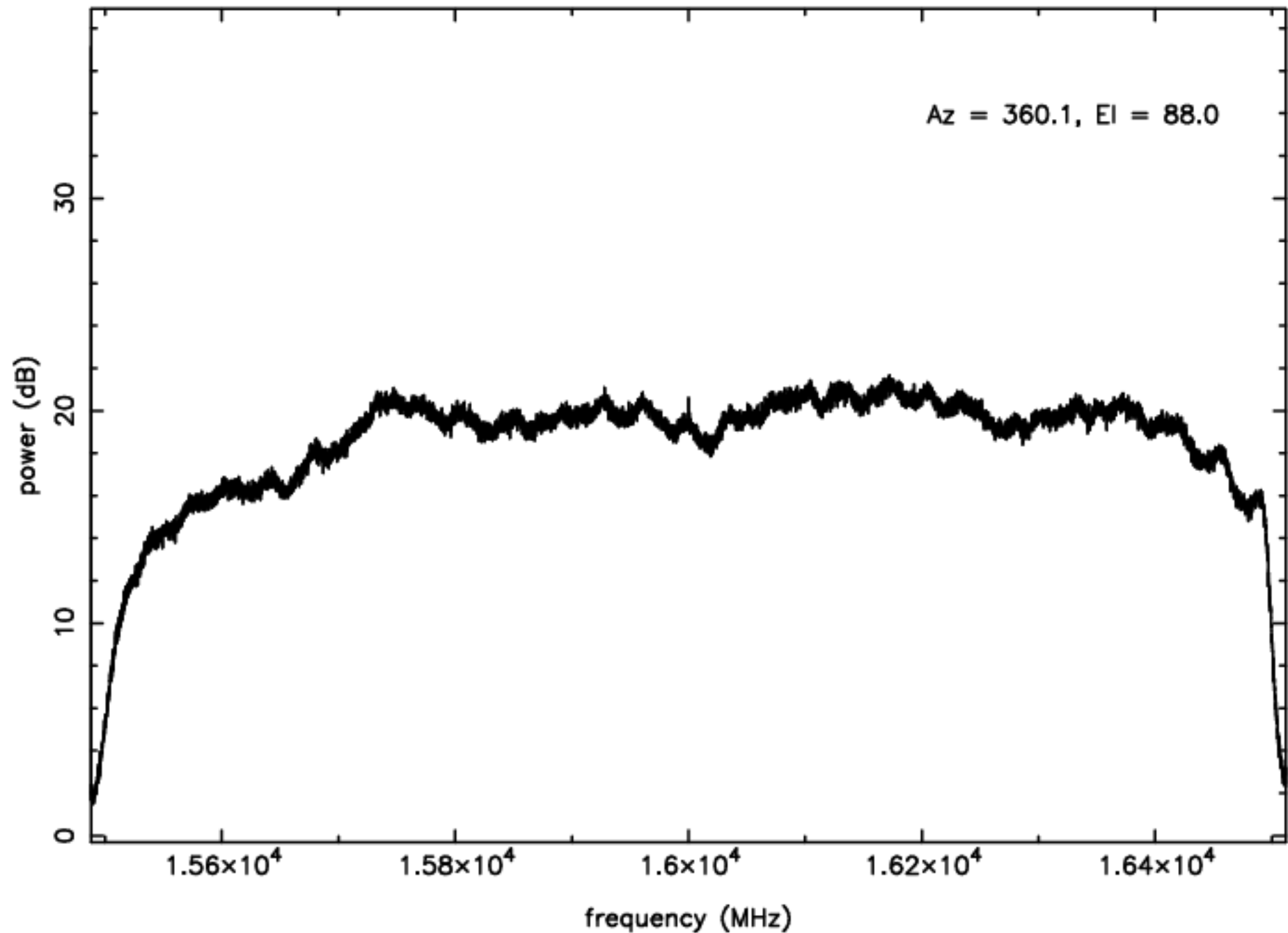
Ku-band RFI plot (mean power) - IF D - ea24
