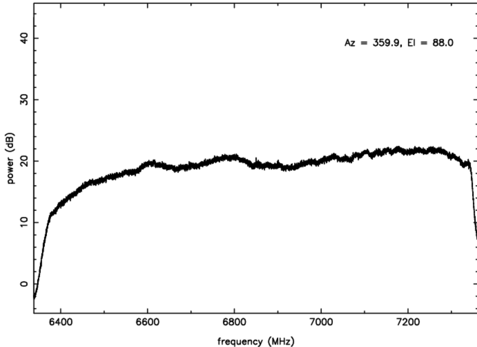
C-band RFI plot (mean power) – IF B – ea24
