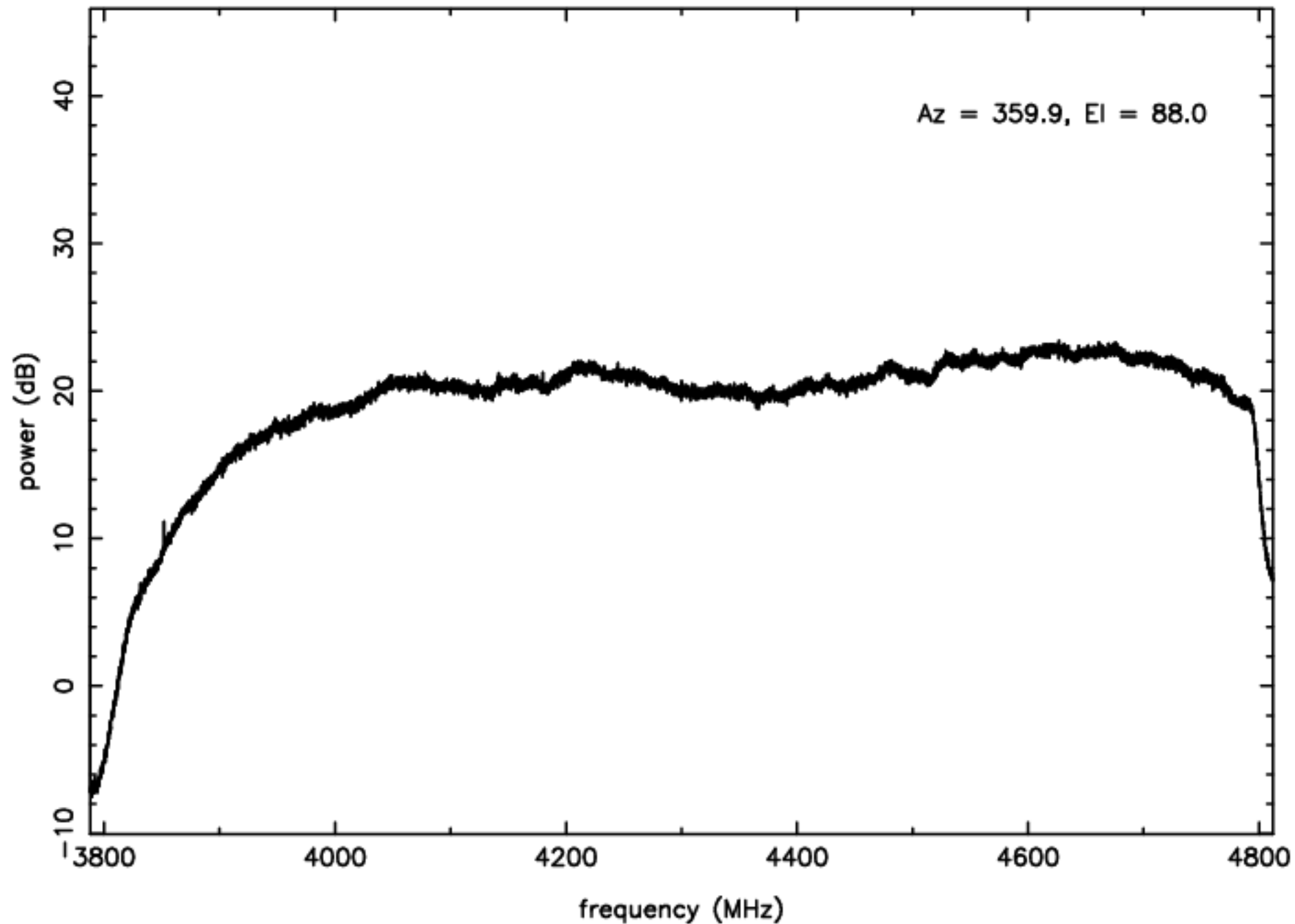
C-band RFI plot (mean power) – IF B – ea24
