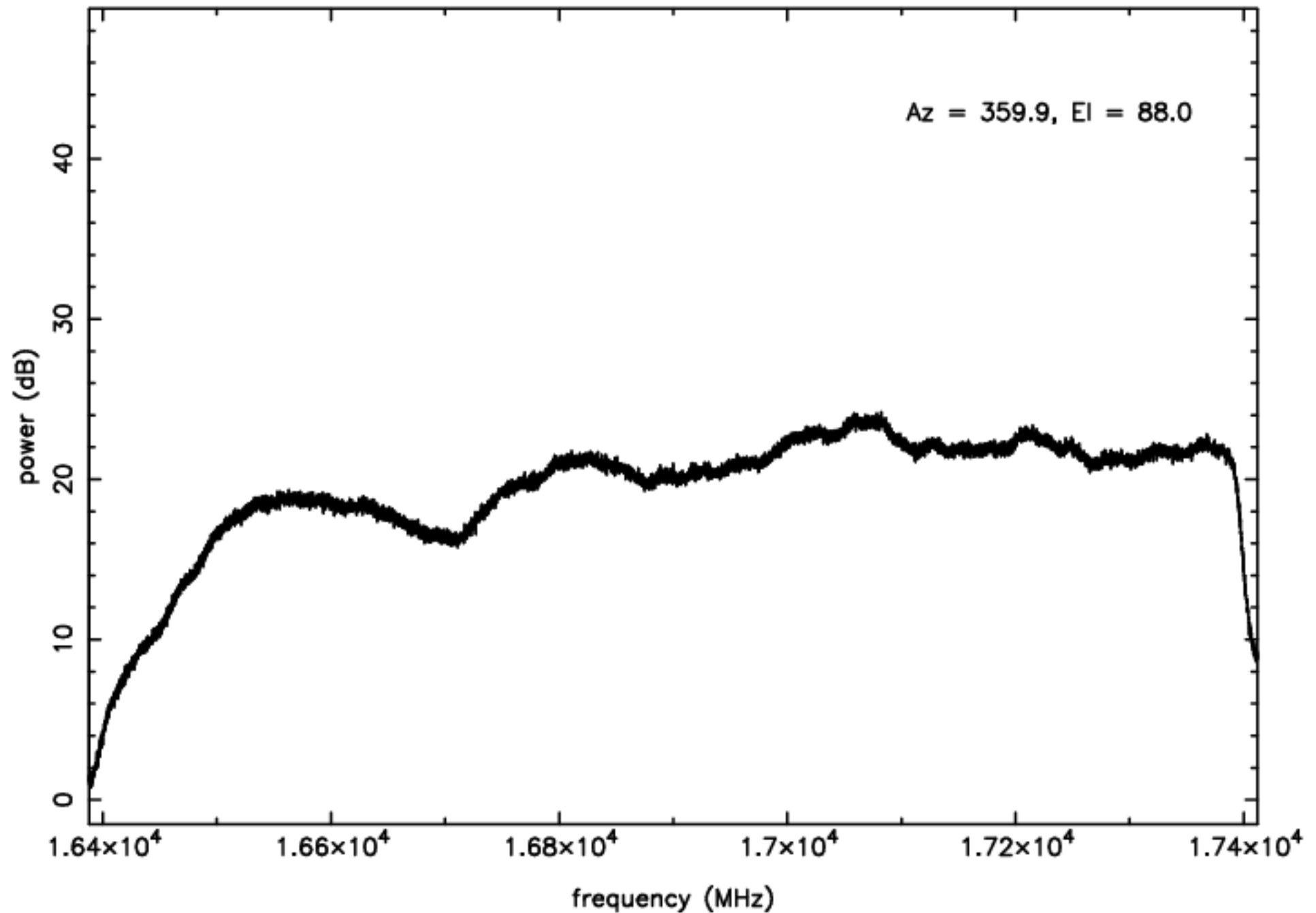
Ku-band RFI plot (mean power) - IF D - ea10
