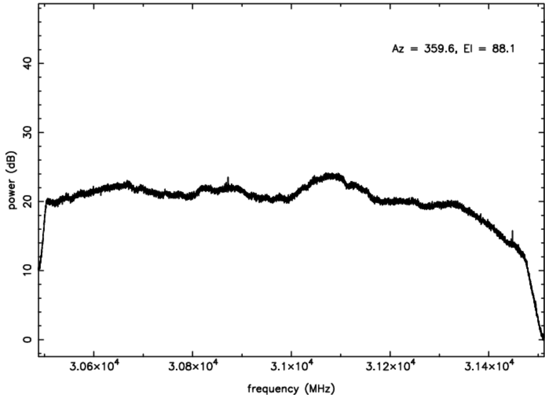
Ka-band RFI plot (mean power) – IF B – ea10
