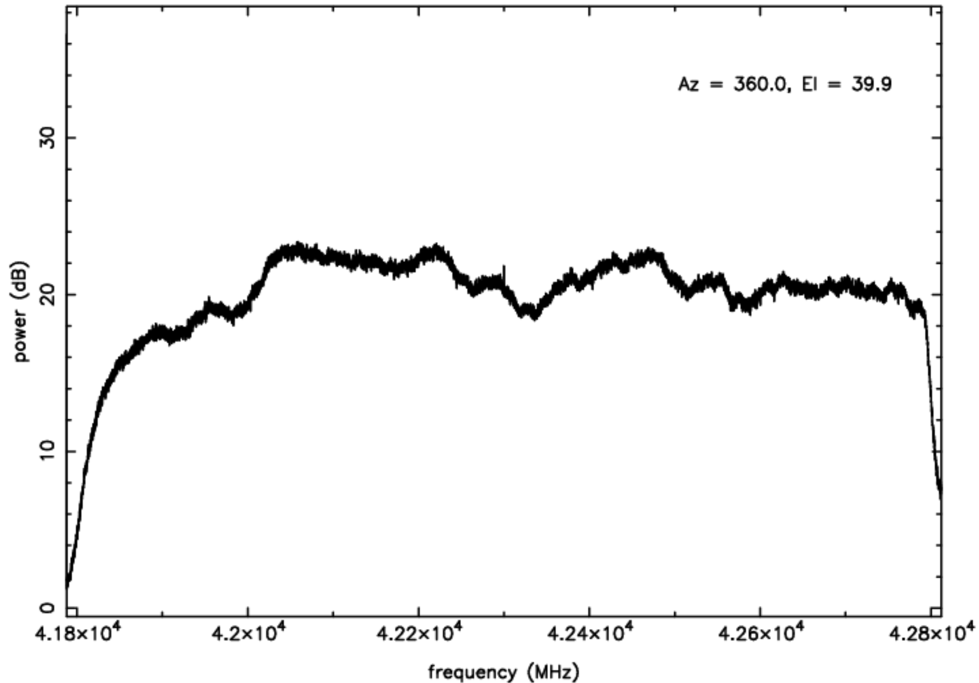
Q-band RFI plot (mean power) – IF D – ea24
