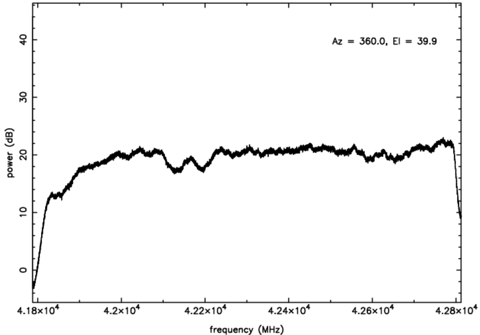
Q-band RFI plot (mean power) - IF B - ea24
