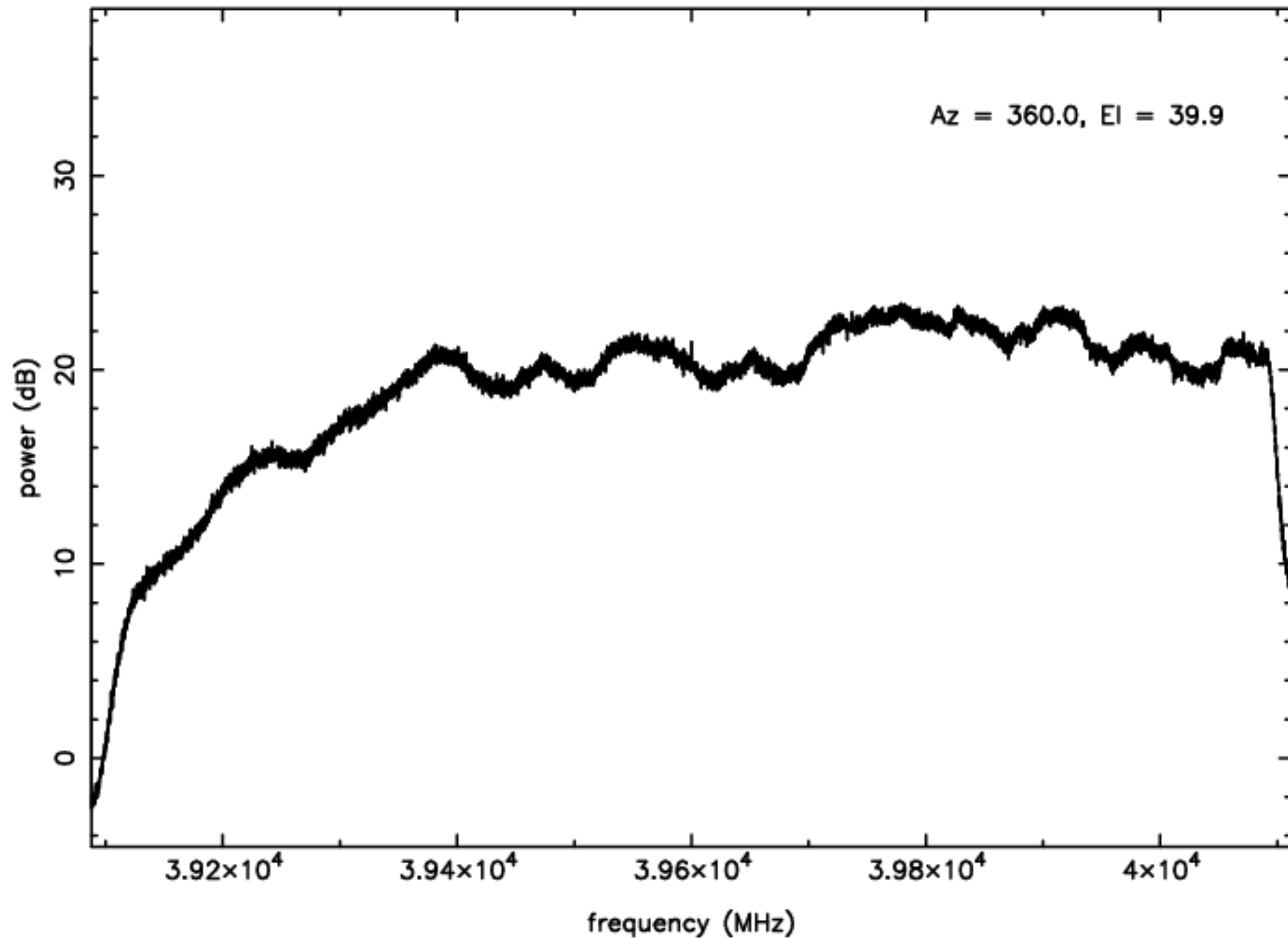
Q-band RFI plot (mean power) – IF D – ea24
