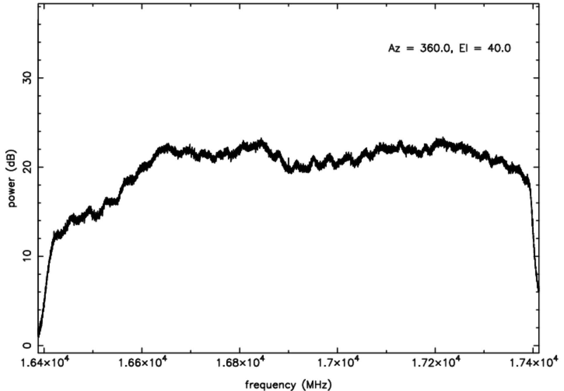
Ku-band RFI plot (mean power) – IF D – ea24
