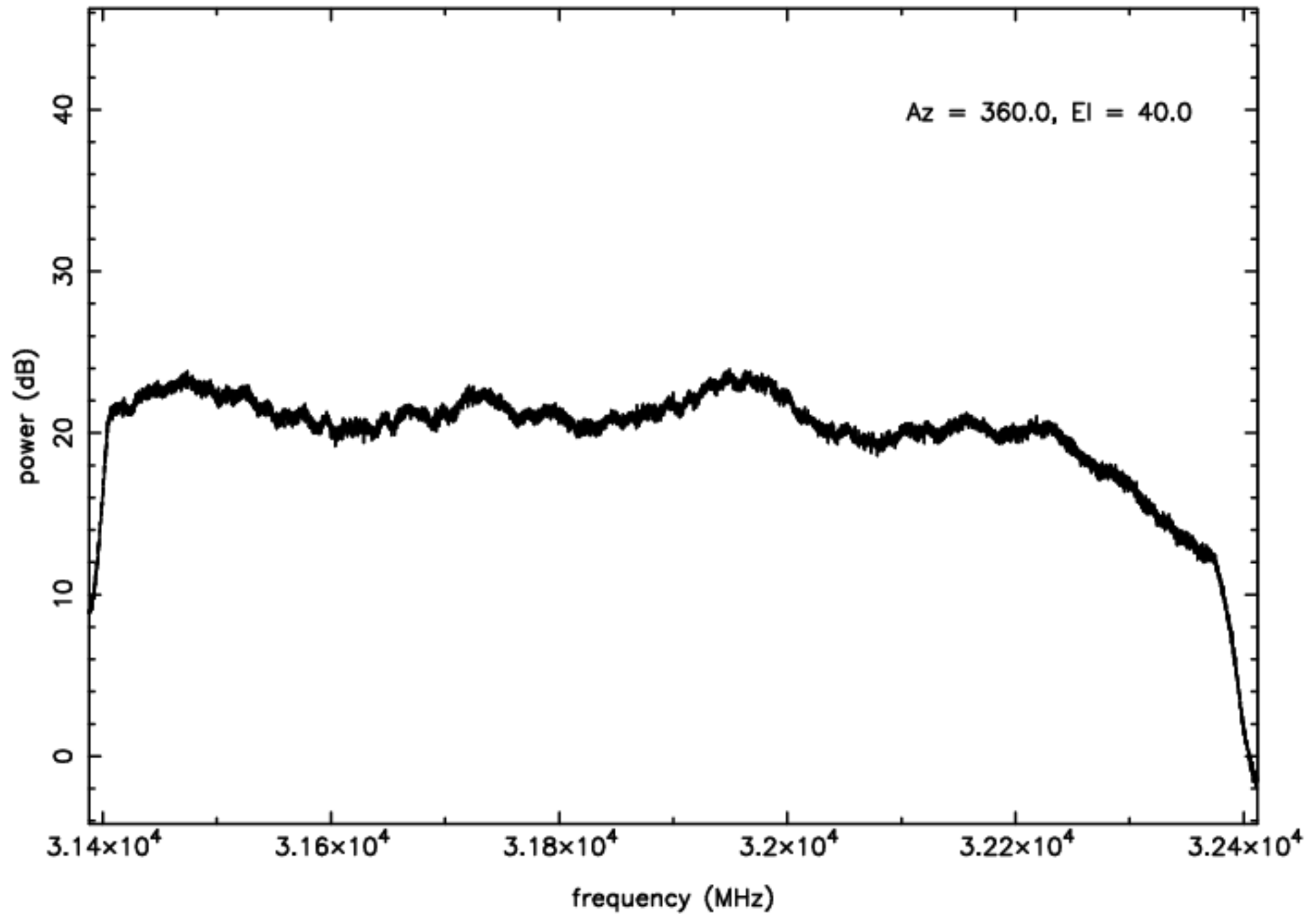
Ka-band RFI plot (mean power) - IF B - ea24
