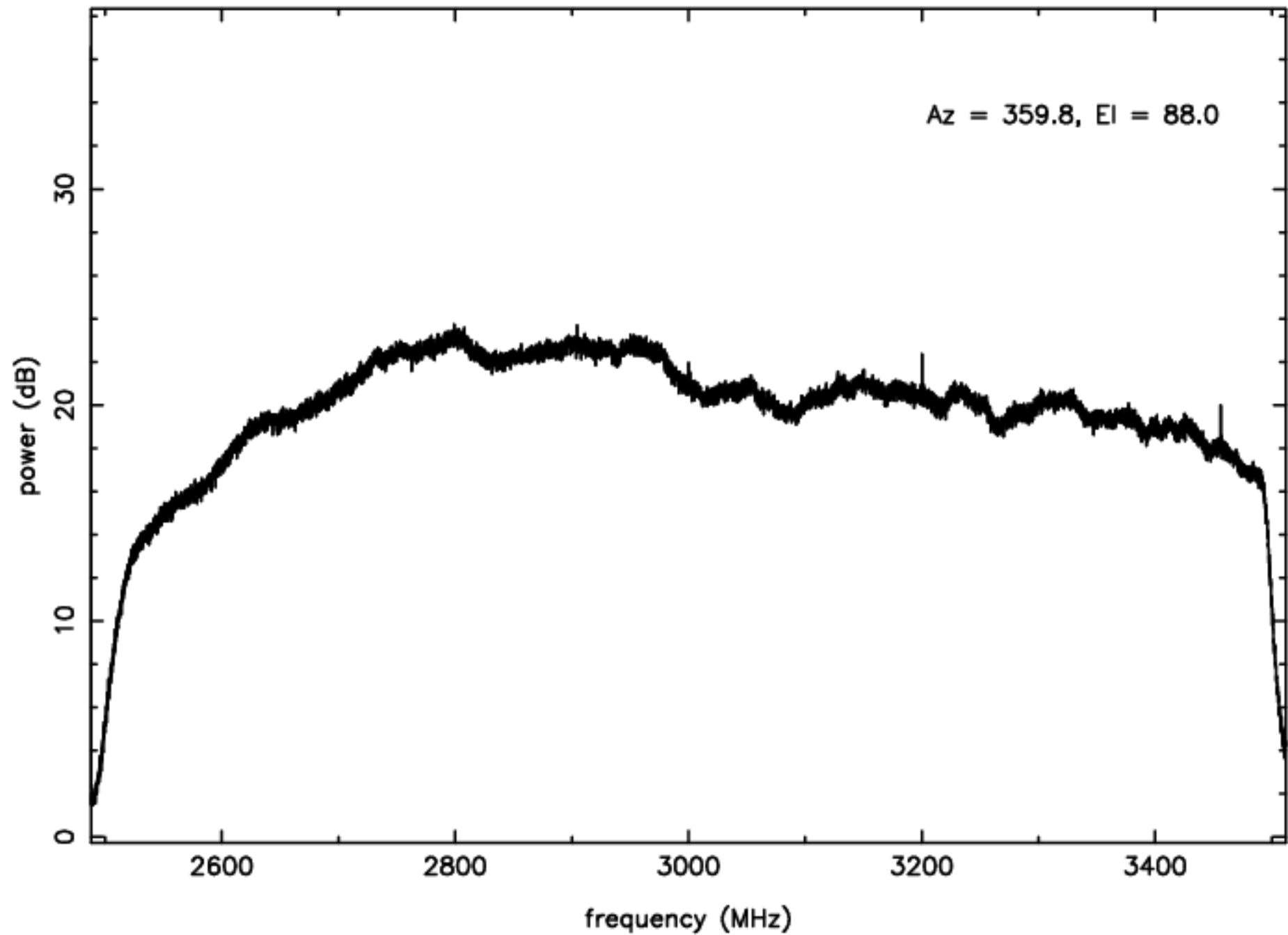
S-band RFI plot (mean power) – IF D – ea24
