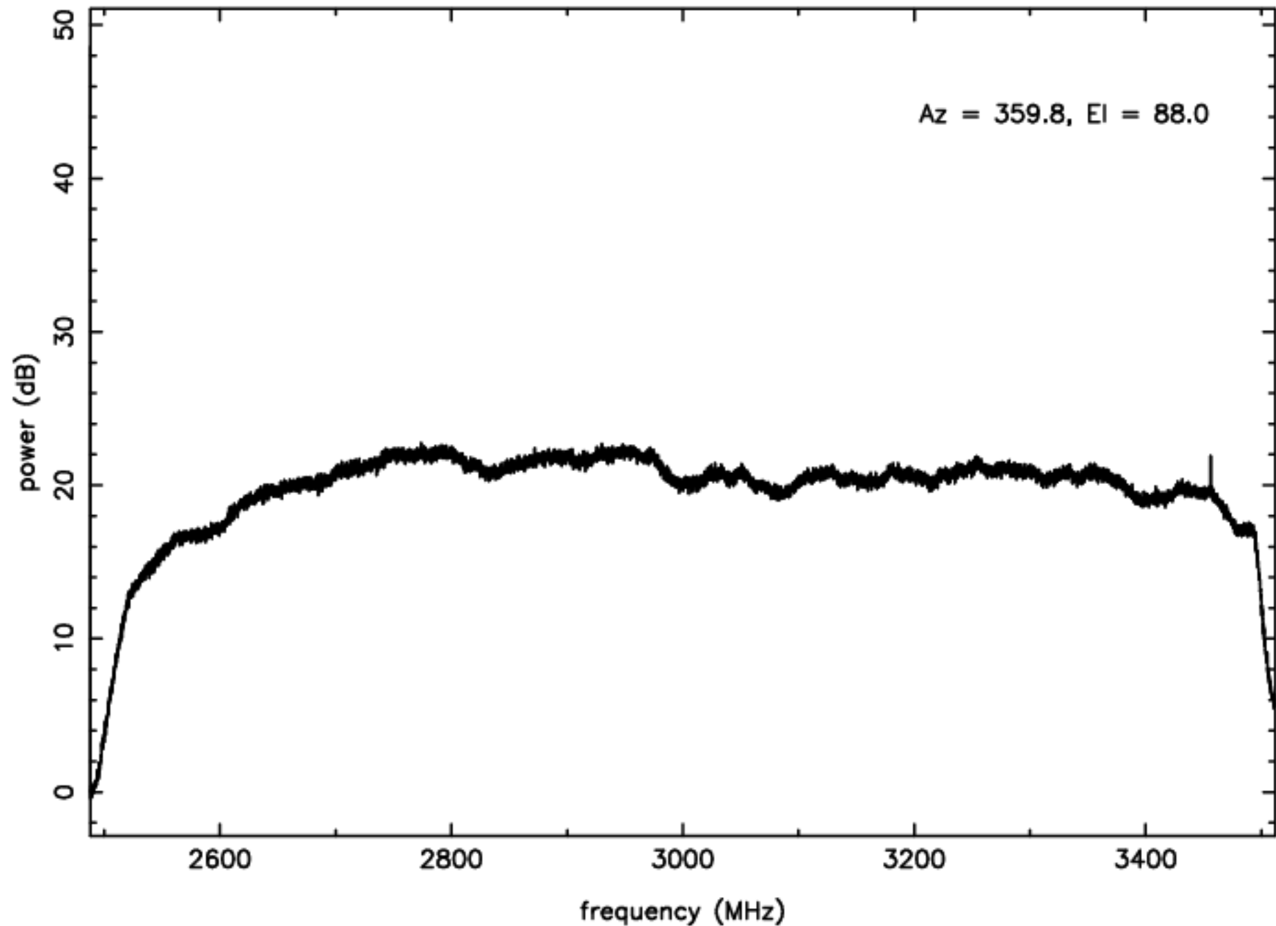
S-band RFI plot (mean power) – IF B – ea24
