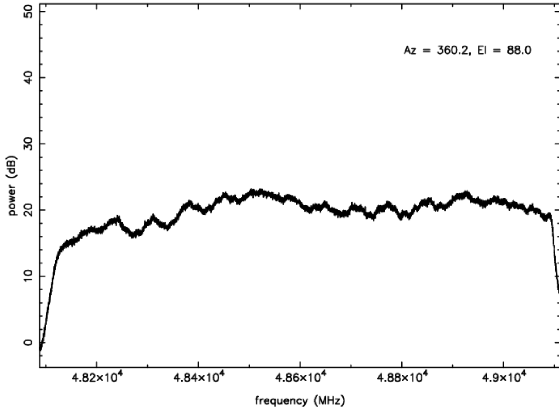
Q-band RFI plot (mean power) – IF B – ea24
