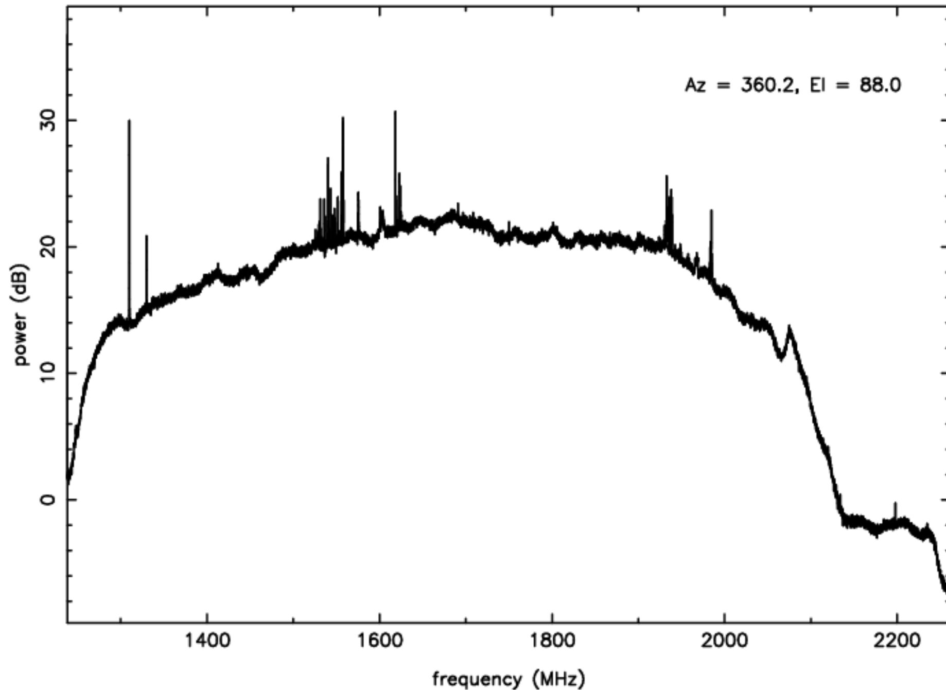
L-band RFI plot (mean power) – IF D – ea24
