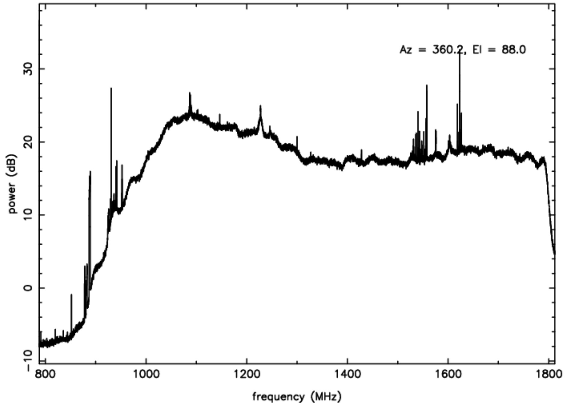
L-band RFI plot (mean power) – IF D – ea24
