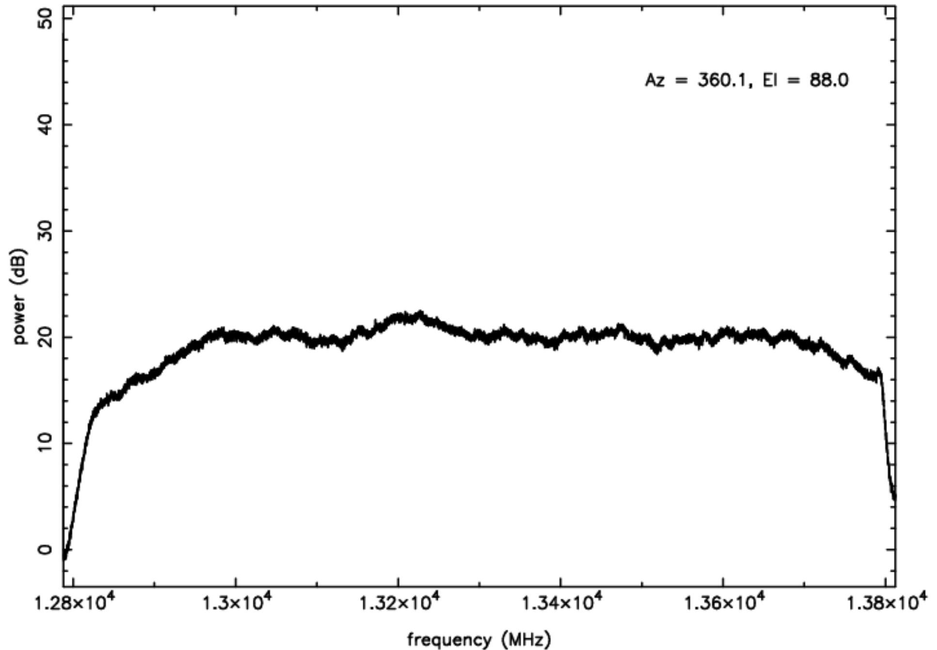
Ku-band RFI plot (mean power) - IF B - ea24
