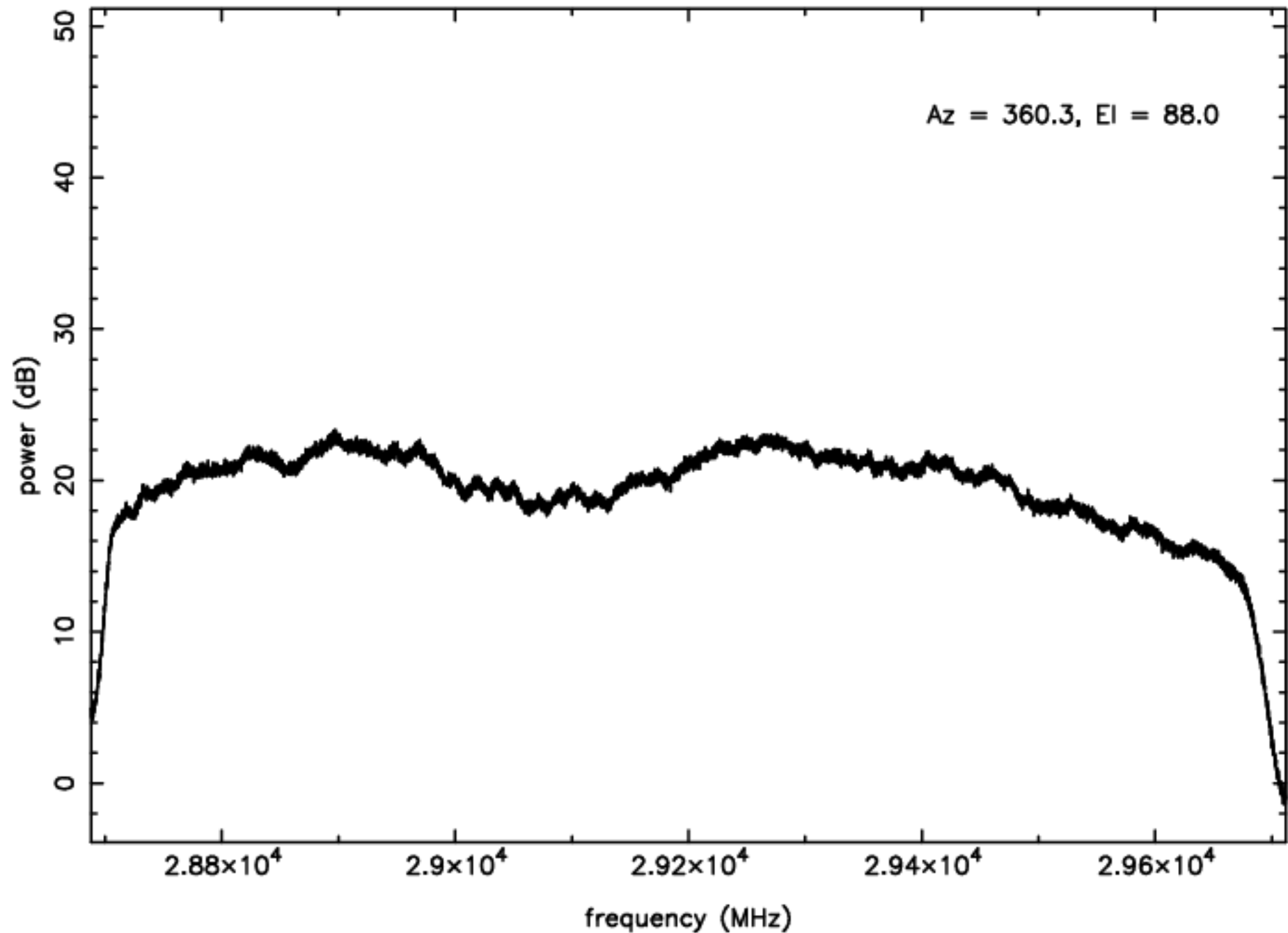
Ka-band RFI plot (mean power) – IF B – ea24
