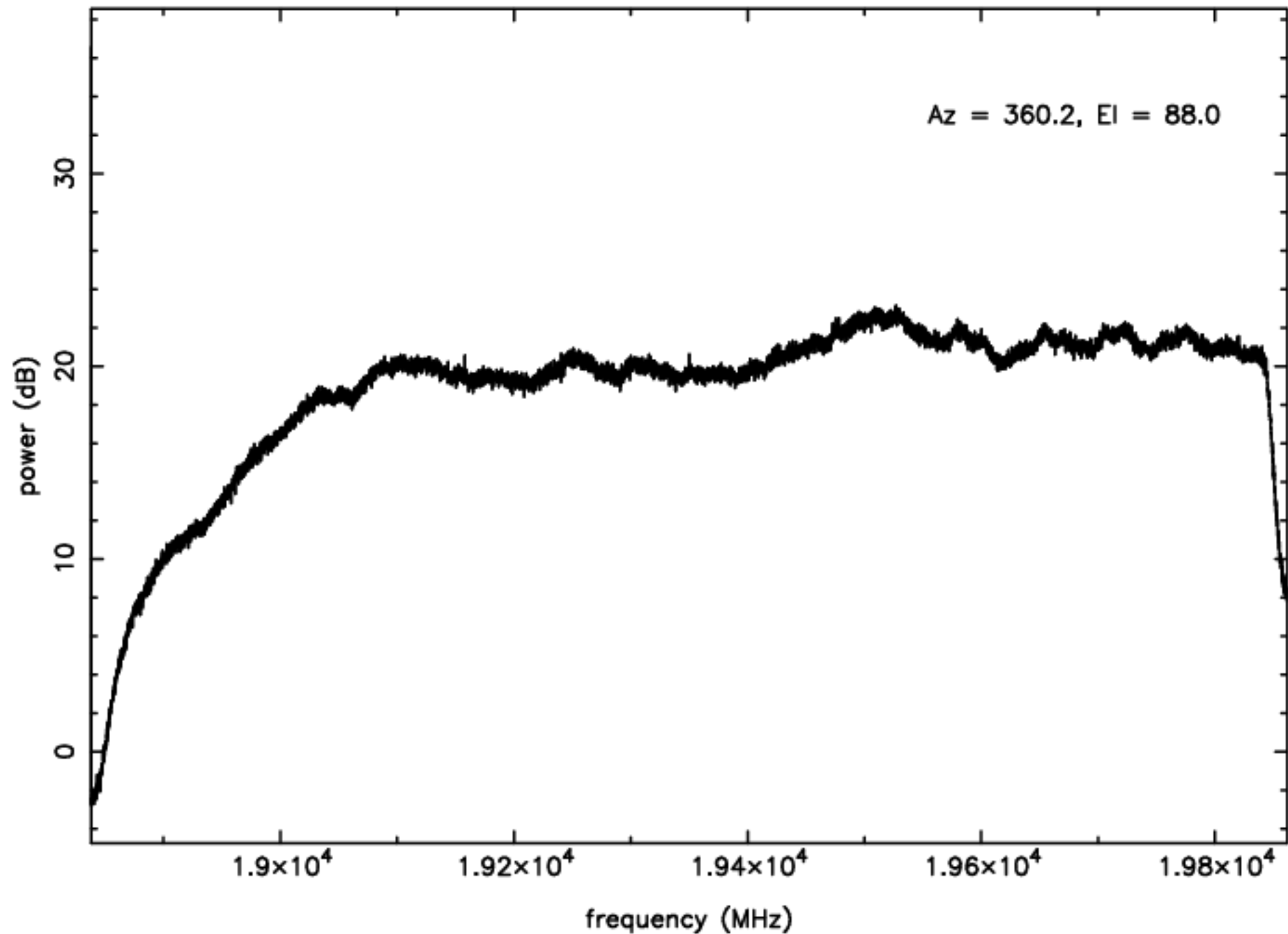
K-band RFI plot (mean power) – IF D – ea24
