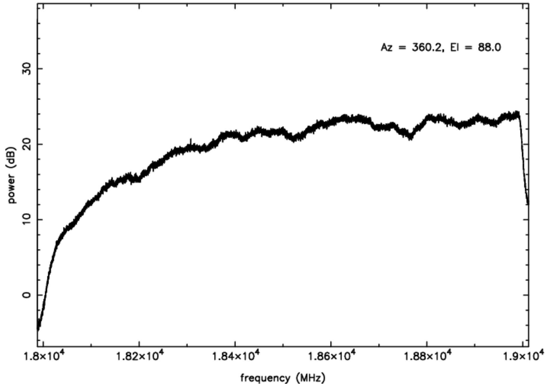
K-band RFI plot (mean power) – IF D – ea24
