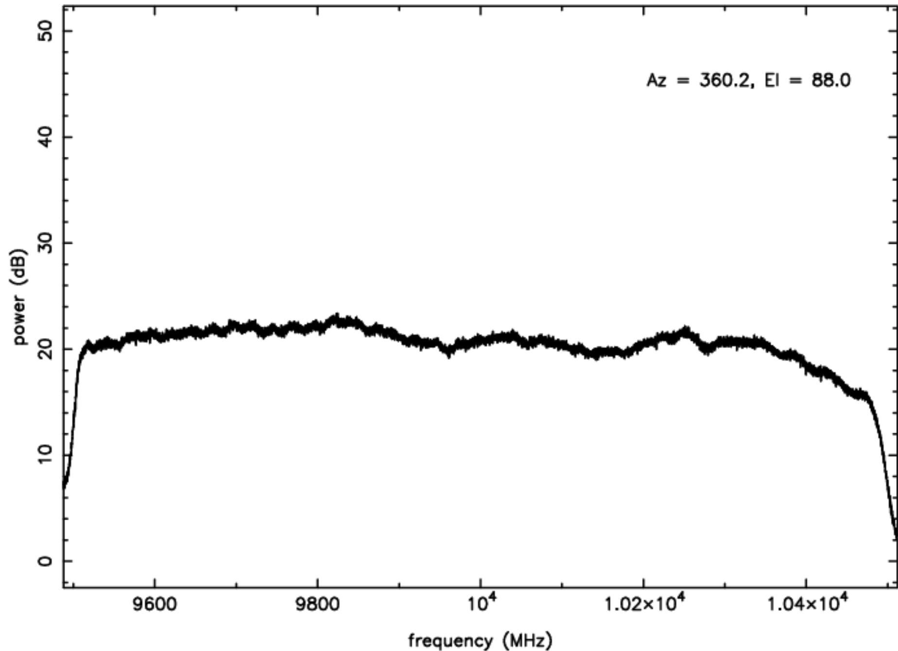
X-band RFI plot (mean power) – IF D – ea14
