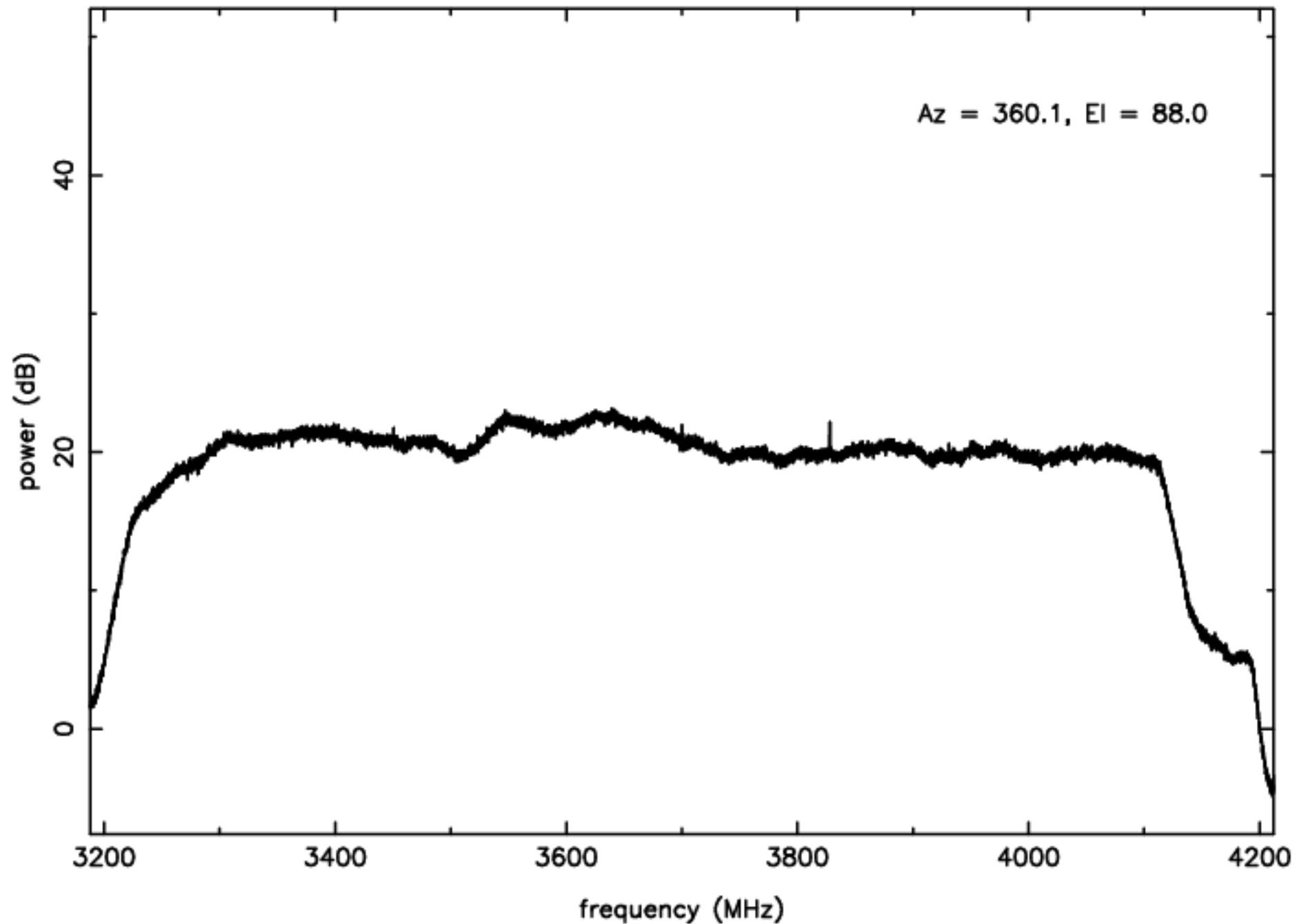
S-band RFI plot (mean power) – IF B – ea14
