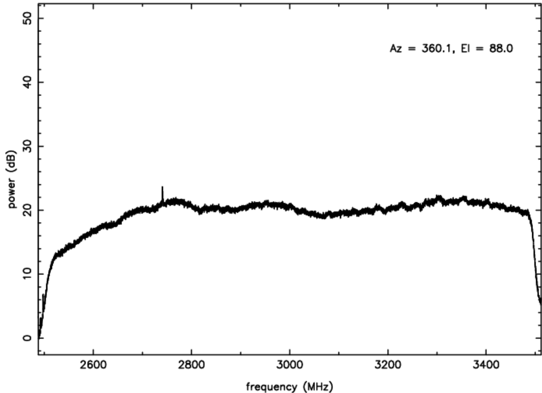
S-band RFI plot (mean power) – IF D – ea14
