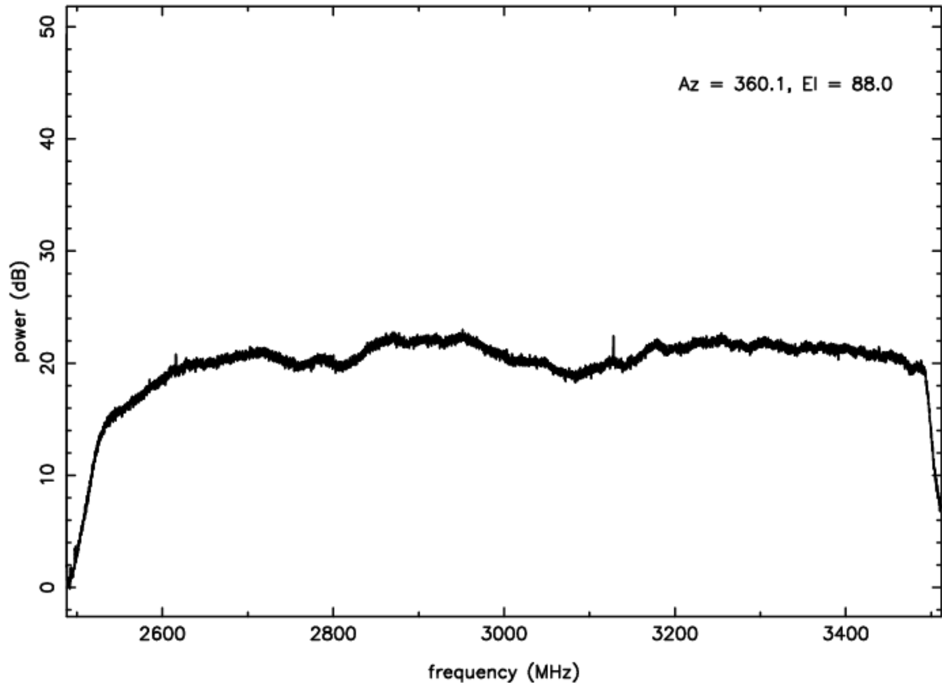
S-band RFI plot (mean power) – IF B – ea14
