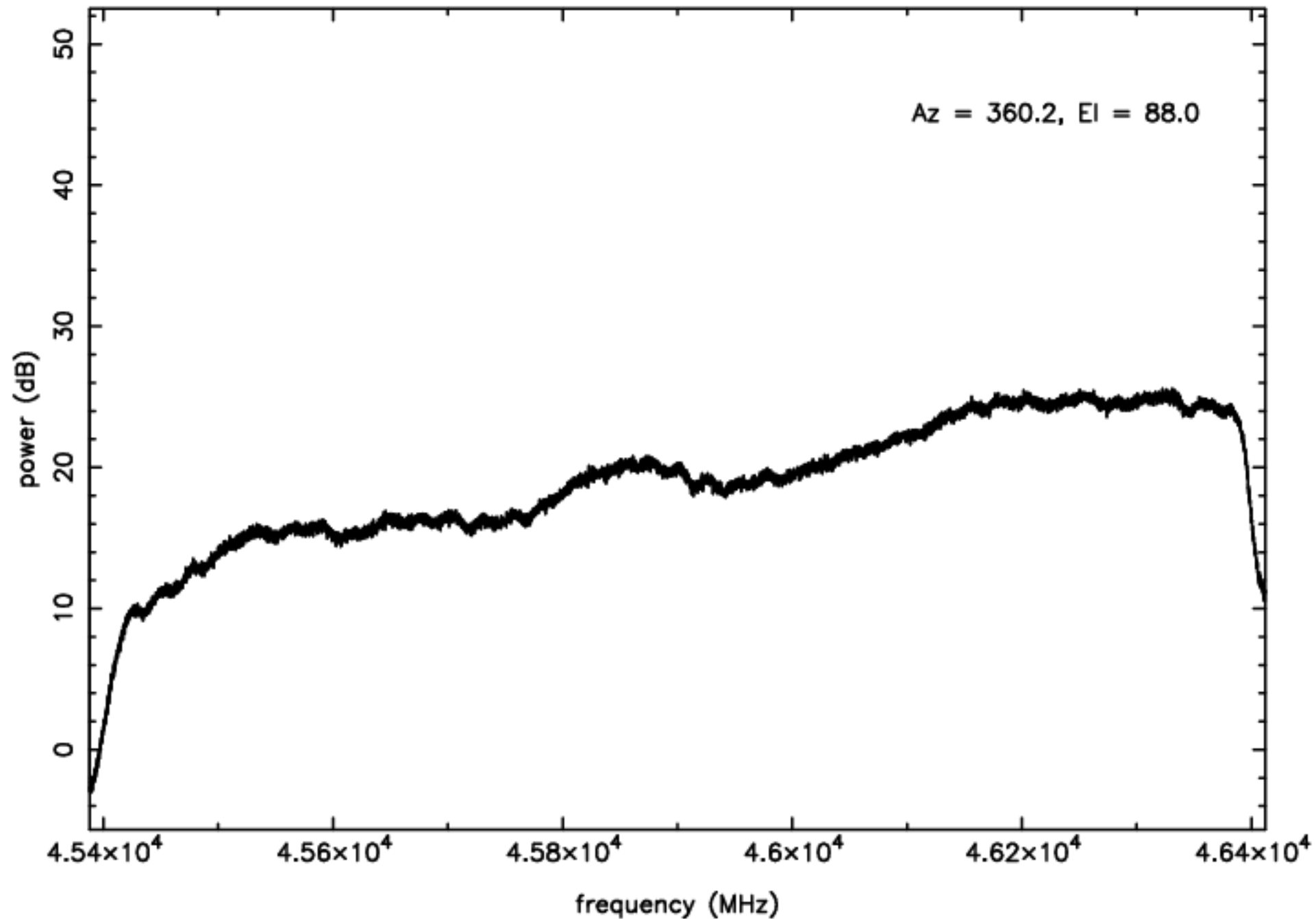
Q-band RFI plot (mean power) – IF D – ea14
