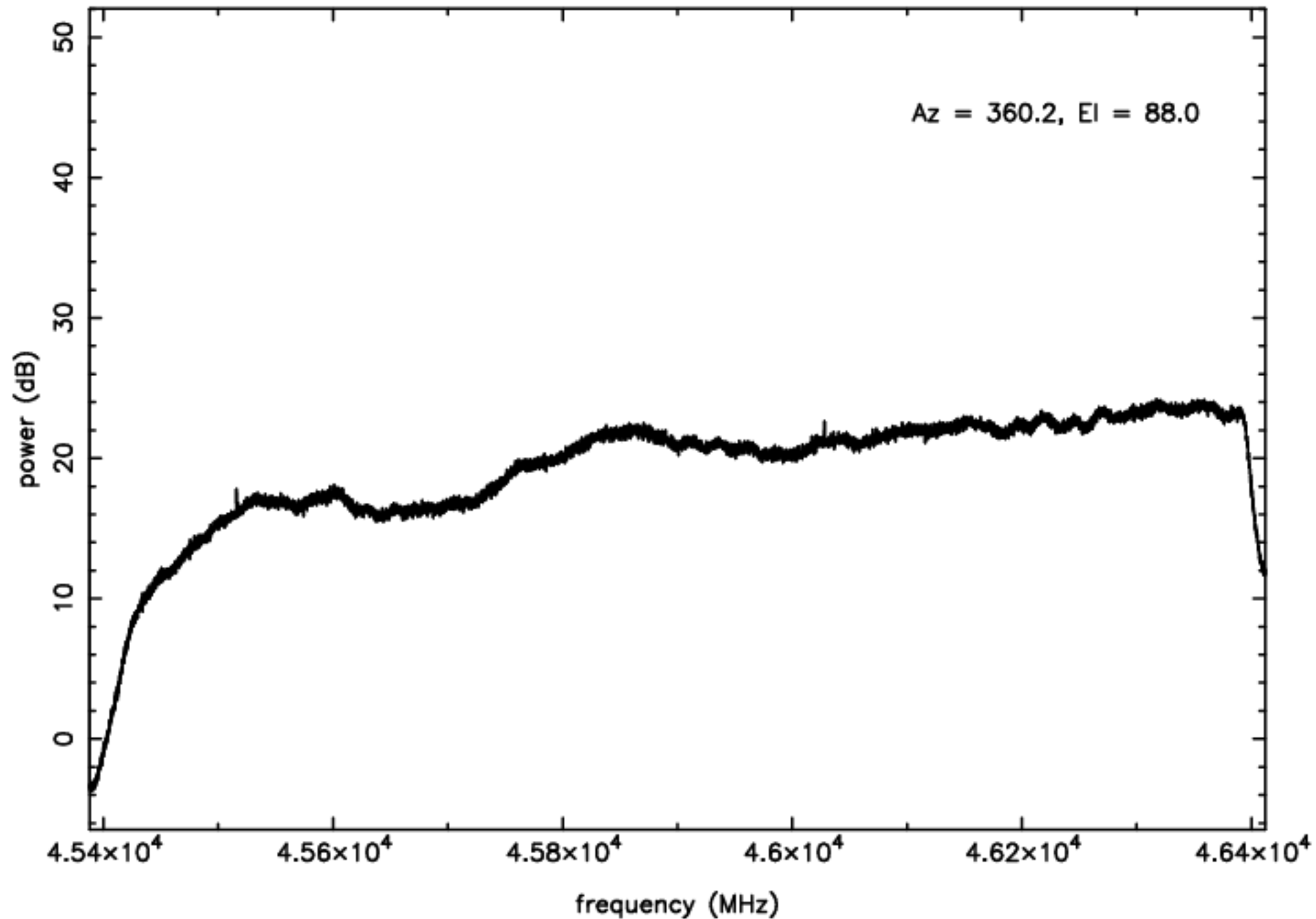
Q-band RFI plot (mean power) – IF B – ea14
