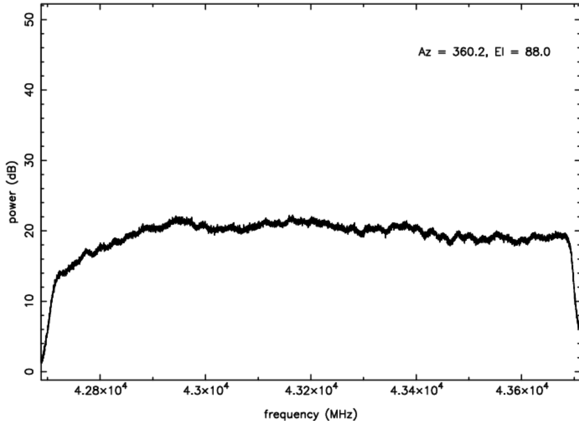
Q-band RFI plot (mean power) – IF D – ea14
