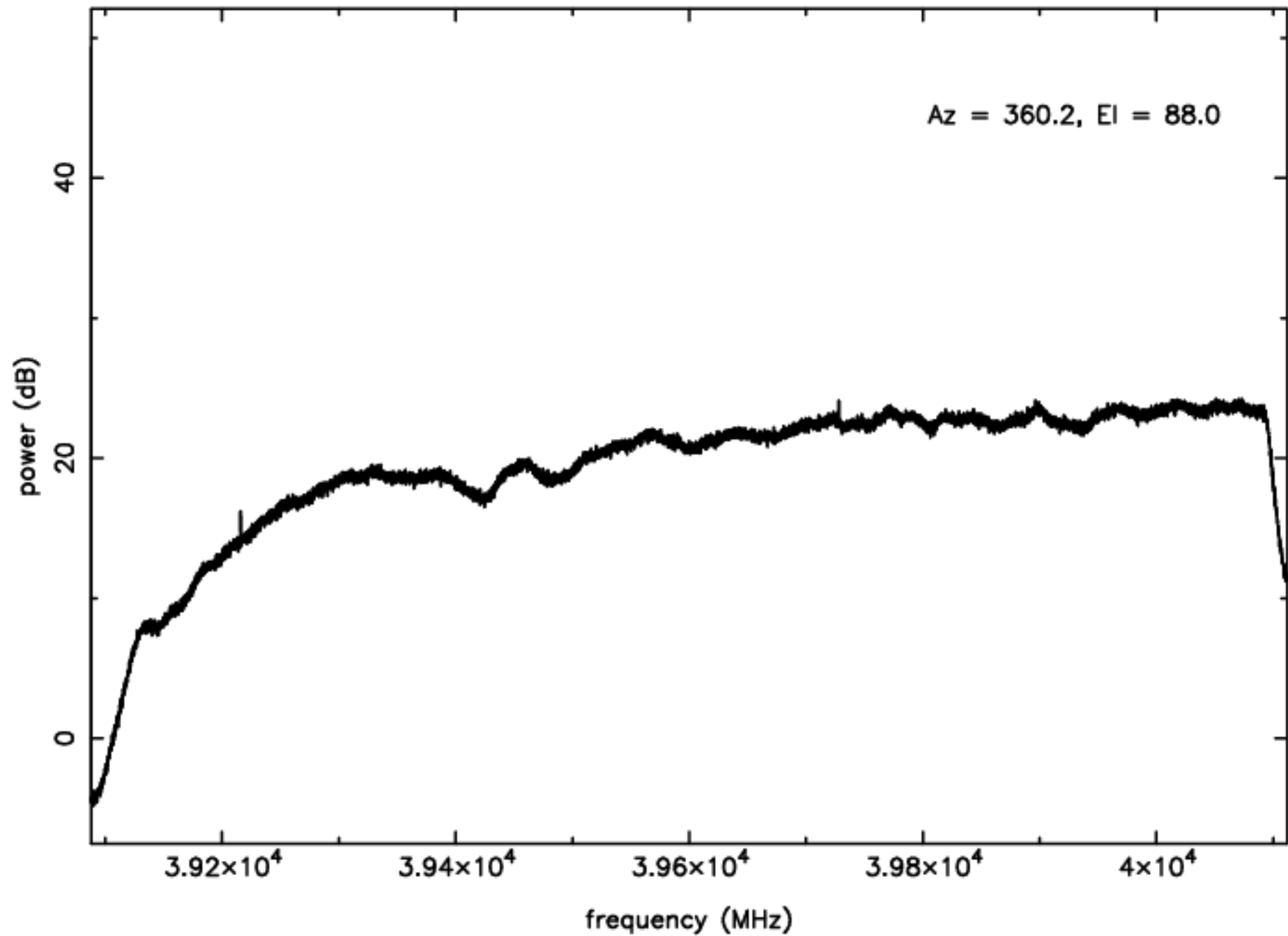
Q-band RFI plot (mean power) - IF B - ea14
