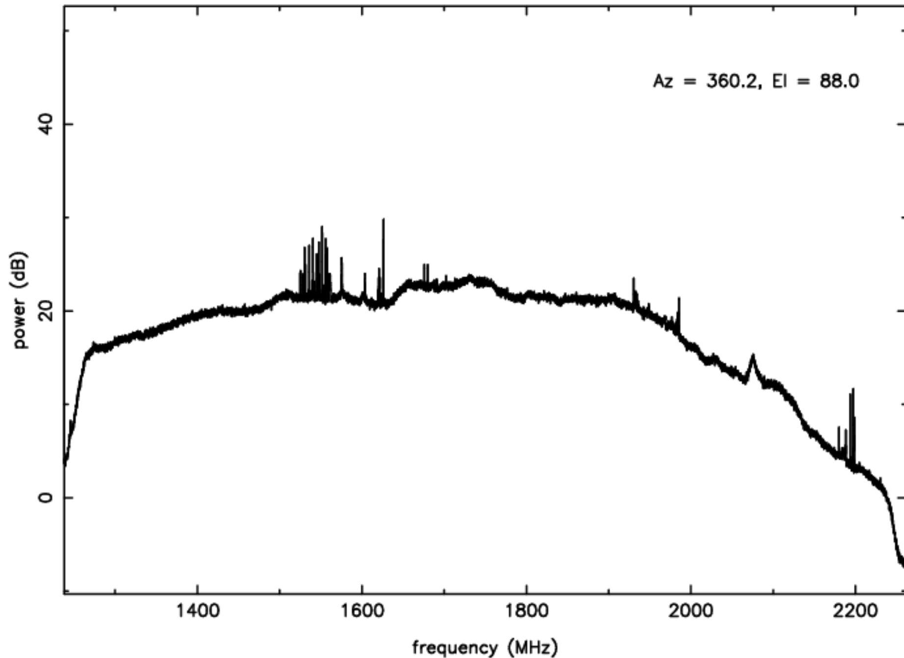
L-band RFI plot (mean power) – IF D – ea14
