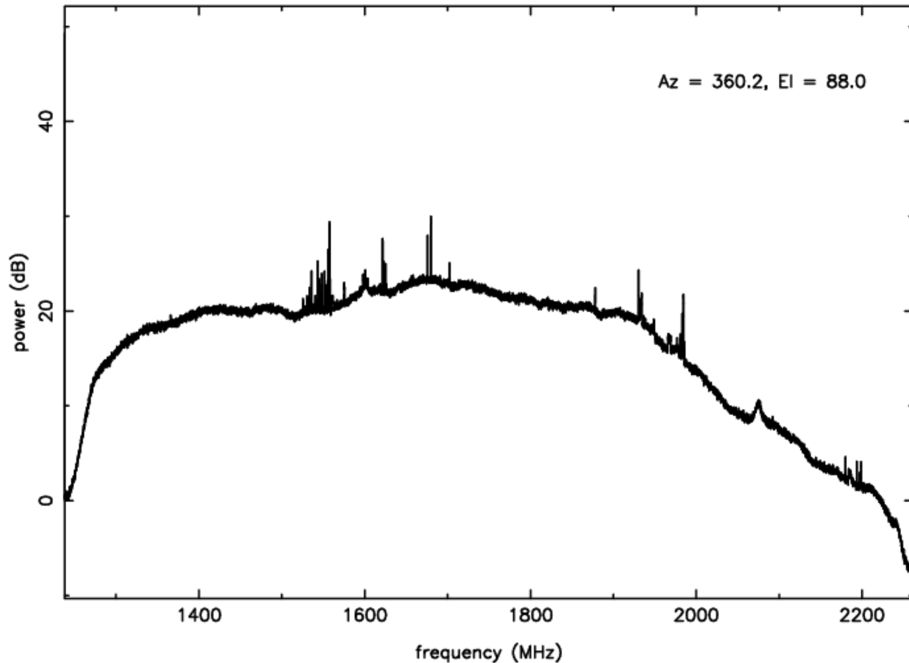
L-band RFI plot (mean power) – IF B – ea14
