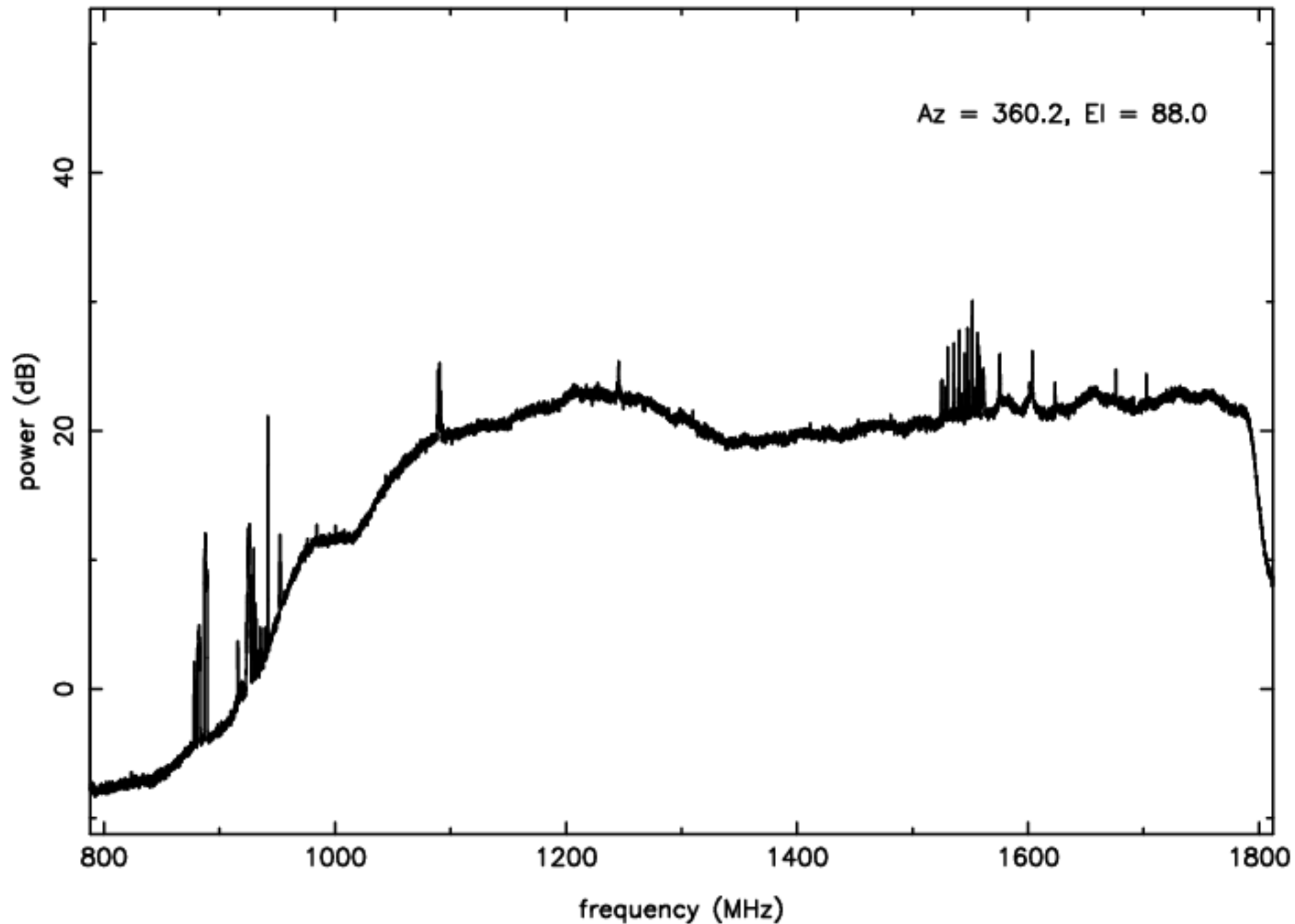
L-band RFI plot (mean power) – IF D – ea14
