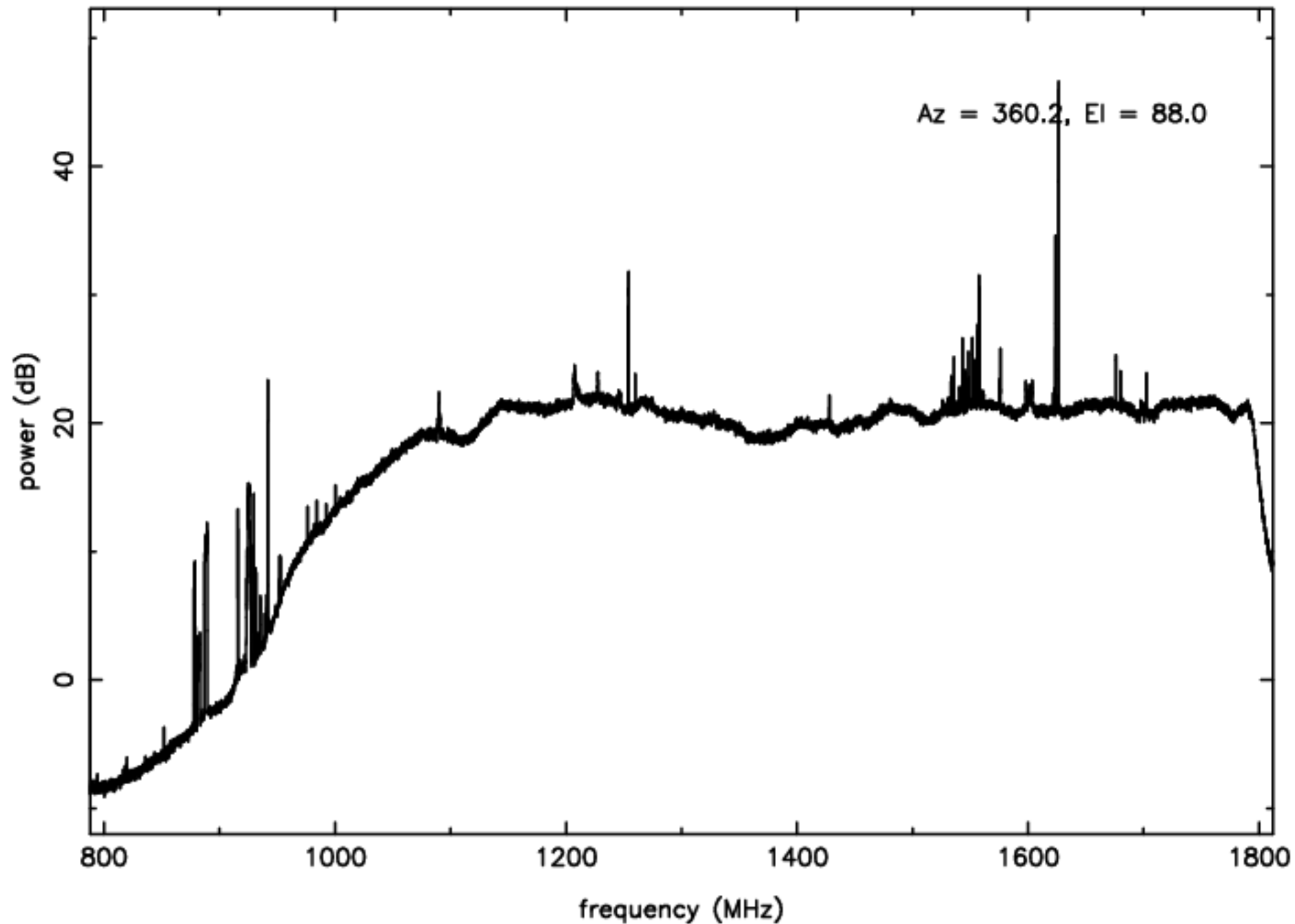
L-band RFI plot (mean power) – IF B – ea14
