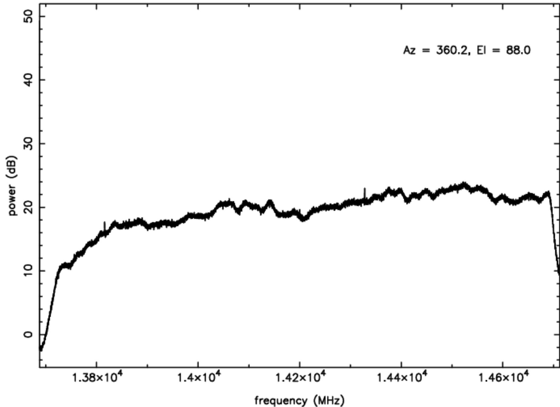
Ku-band RFI plot (mean power) - IF B - ea14
