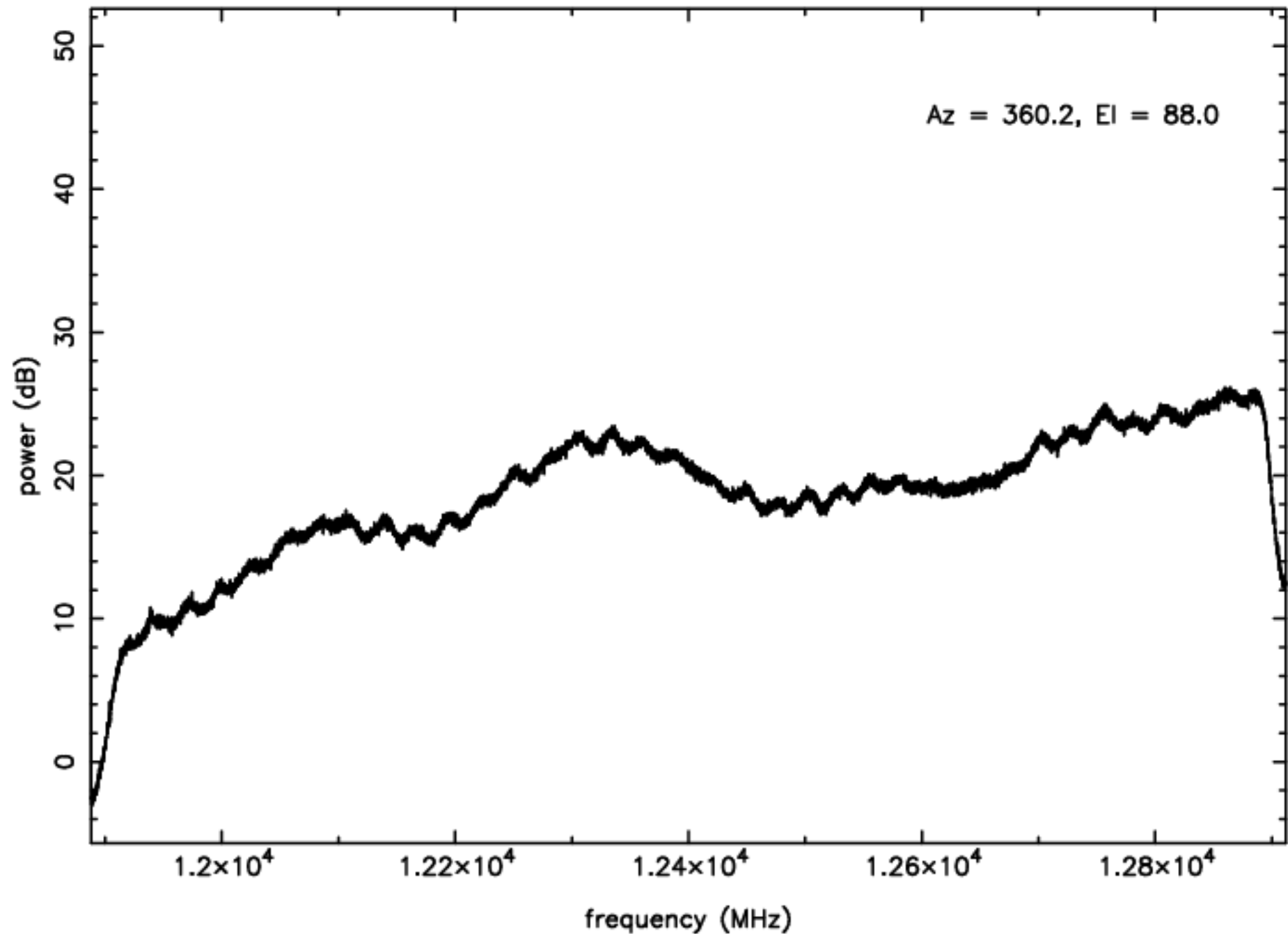
Ku-band RFI plot (mean power) - IF D - ea14
