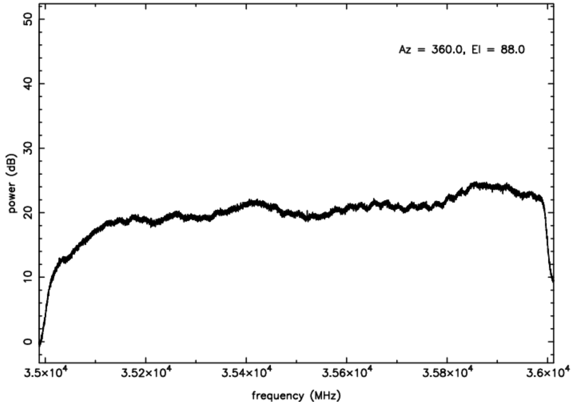
Ka-band RFI plot (mean power) - IF D - ea14
