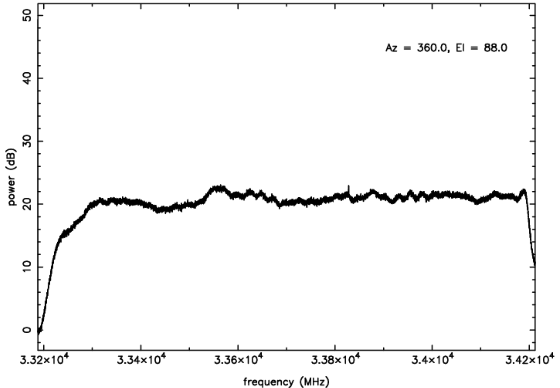
Ka-band RFI plot (mean power) – IF B – ea14
